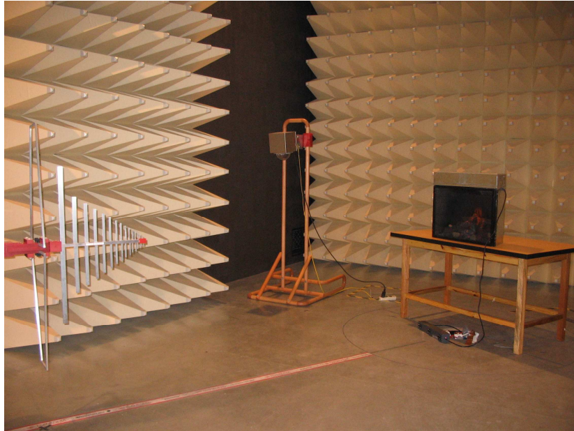
Photograph 2: Set-up for spurious radiated emissions
