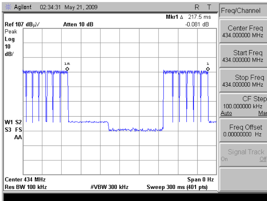
Duty cycle 1
