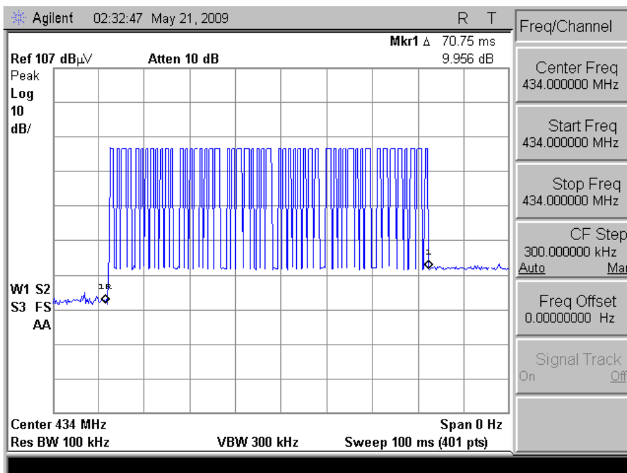
Duty cycle 2
