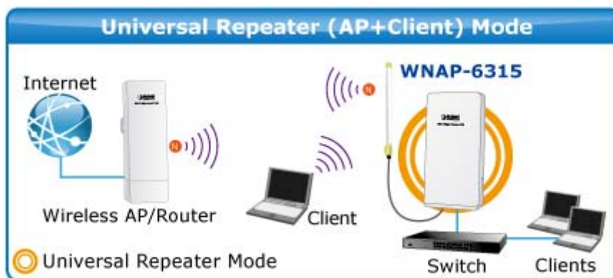
Figure 5-18 Topology – Universal Repeater Mode
