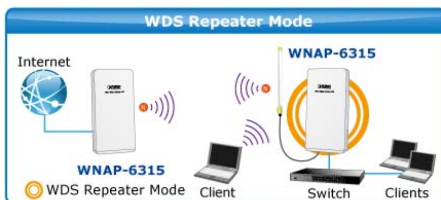
Figure 5-33 Topology – WDS+AP Mode
