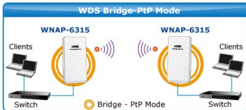
Figure 5-30 Topology – WDS PtP Mode
