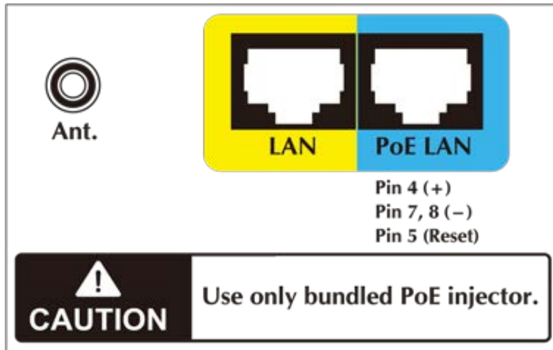
Figure 2-4 Port and Connector Description Label
