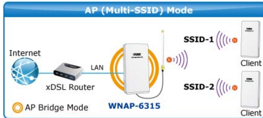
Figure 5-15 Topology – Multiple-SSID Mode
