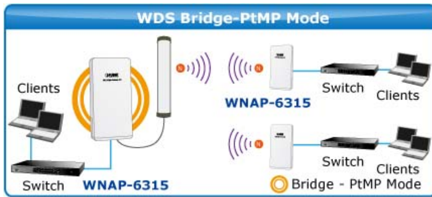
Figure 5-31 Topology – WDS PtMP Mode
