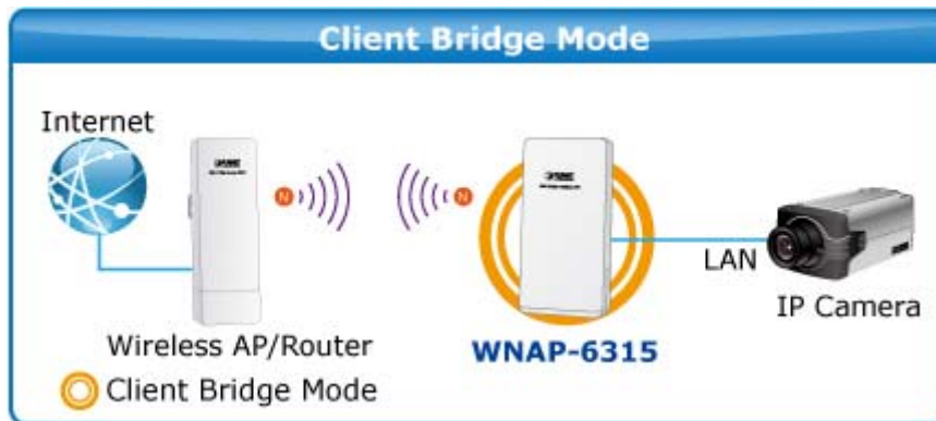
Figure 5-24 Topology – Client Mode
