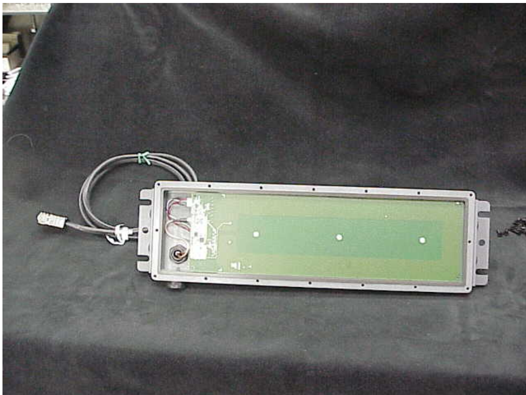
5'x 16' Antenna (Inside)
