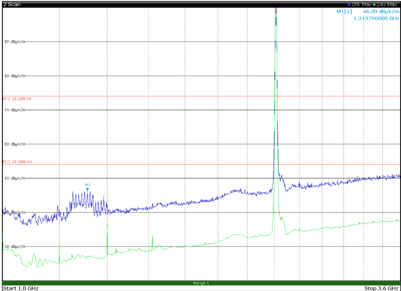
Figure 8.6-4: Radiated spurious emissions 1 to 3.6 GHz, Low channel with antenna in vertical polarization
