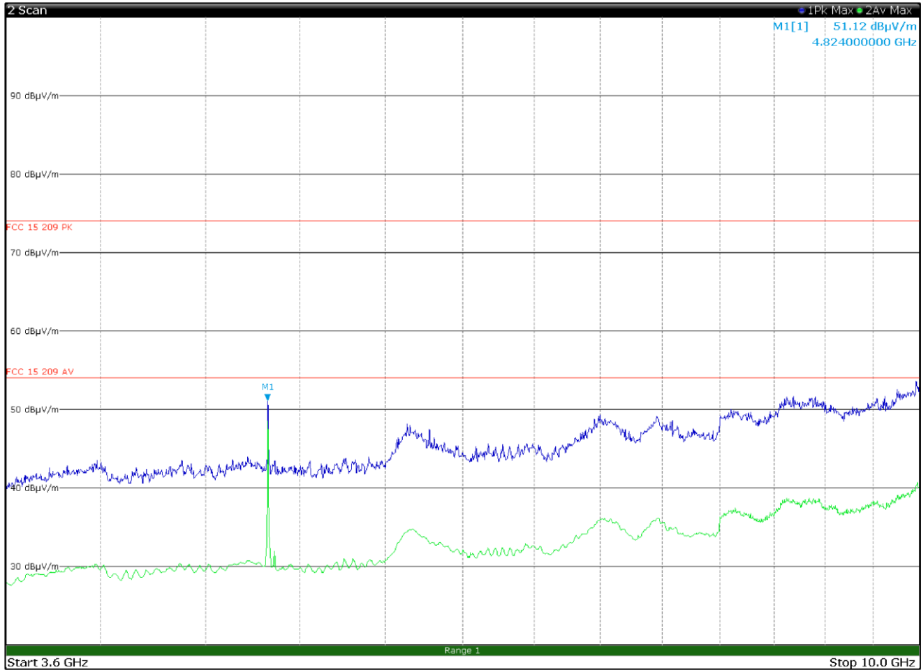
Figure 8.6-9: Radiated spurious emissions 3.6 to 10 GHz, Low channel with antenna in horizontal polarization
