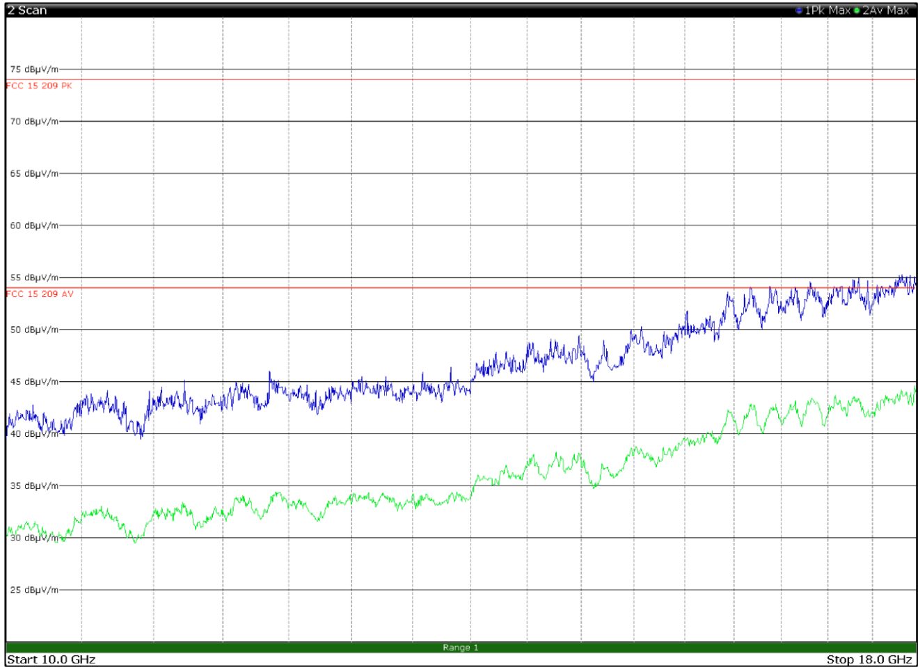
Figure 8.6-15: Radiated spurious emissions 10 to 18 GHz, Low channel with antenna in horizontal polarization
