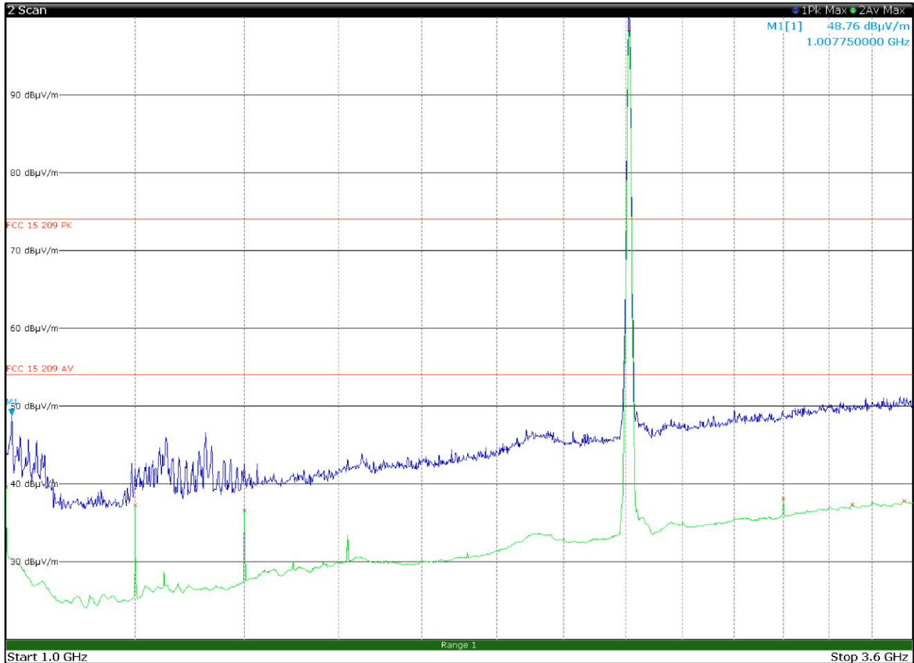
Figure 8.6-3: Radiated spurious emissions 1 to 3.6 GHz, Low channel with antenna in horizontal polarization
