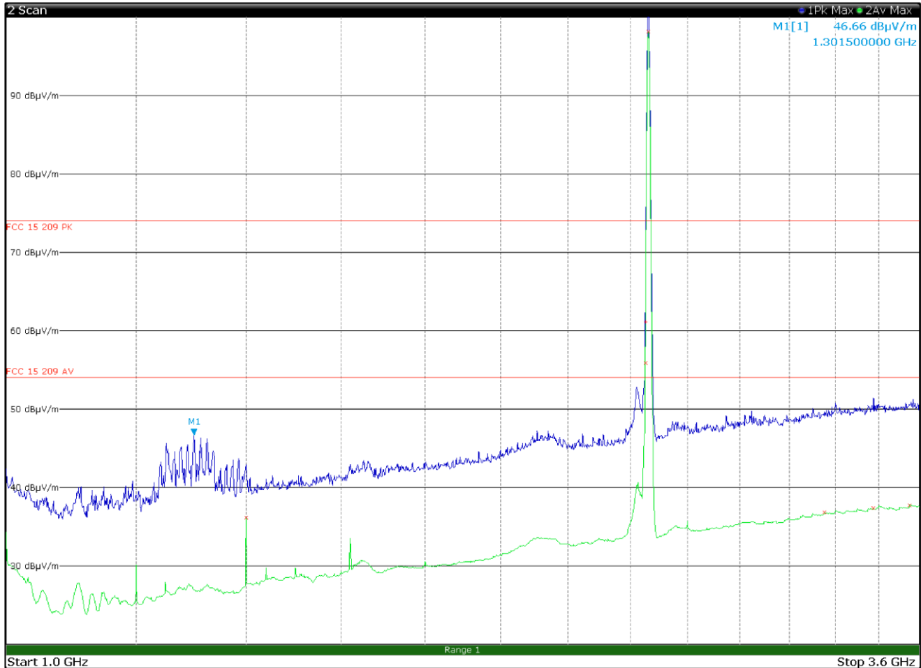
Figure 8.6-8: Radiated spurious emissions 1 to 3.6 GHz, High channel with antenna in vertical polarization
