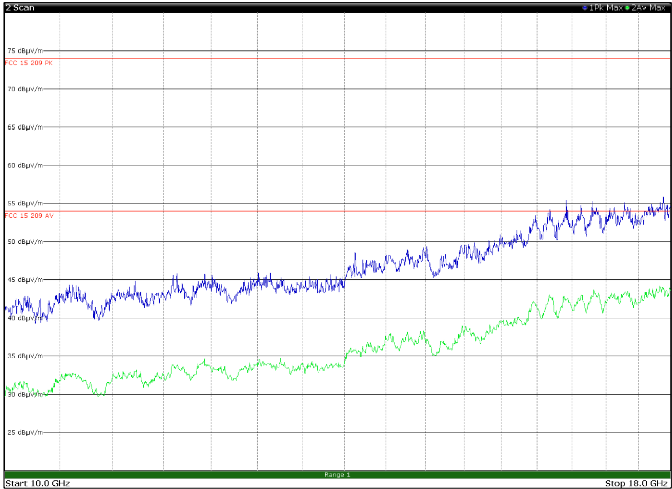
Figure 8.6-20: Radiated spurious emissions 10 to 18 GHz, High channel with antenna in vertical polarization
