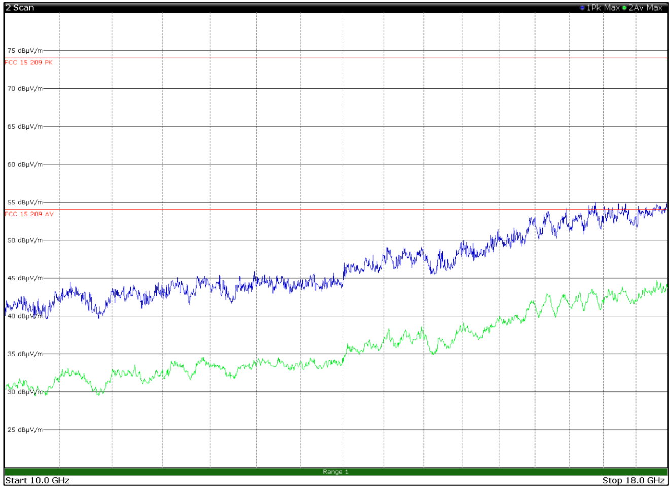
Figure 8.6-17: Radiated spurious emissions 10 to 18 GHz, Mid channel with antenna in horizontal polarization
