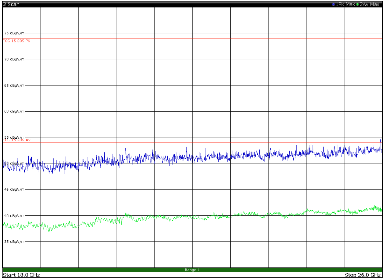
Figure 8.6-22: Radiated spurious emissions 18 to 26 GHz, Low channel with antenna in vertical polarization
