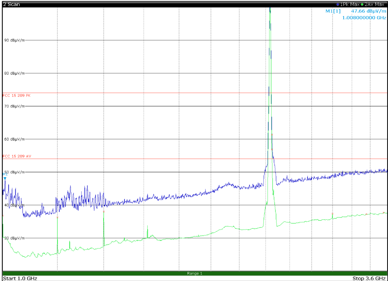
Figure 8.6-5: Radiated spurious emissions 1 to 3.6 GHz, Mid channel with antenna in horizontal polarization
