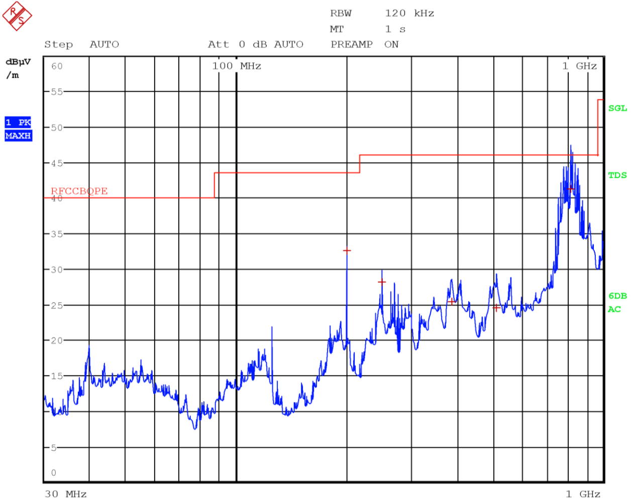
Figure 8.6-1: Radiated spurious emissions 30 to 1000 MHz, Mid channel with antenna in horizontal polarization
