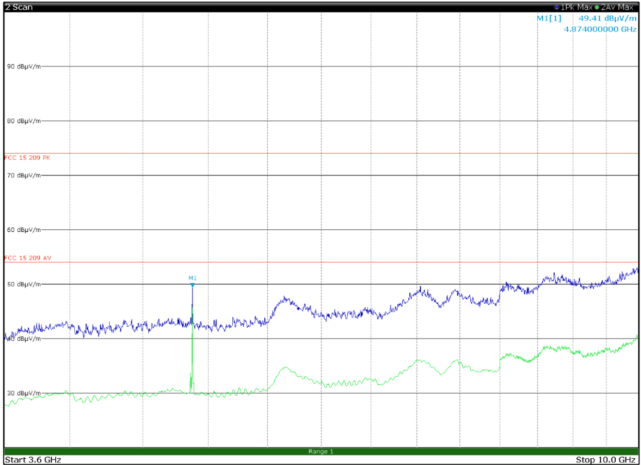
Figure 8.6-11: Radiated spurious emissions 3.6 to 10 GHz, Mid channel with antenna in horizontal polarization
