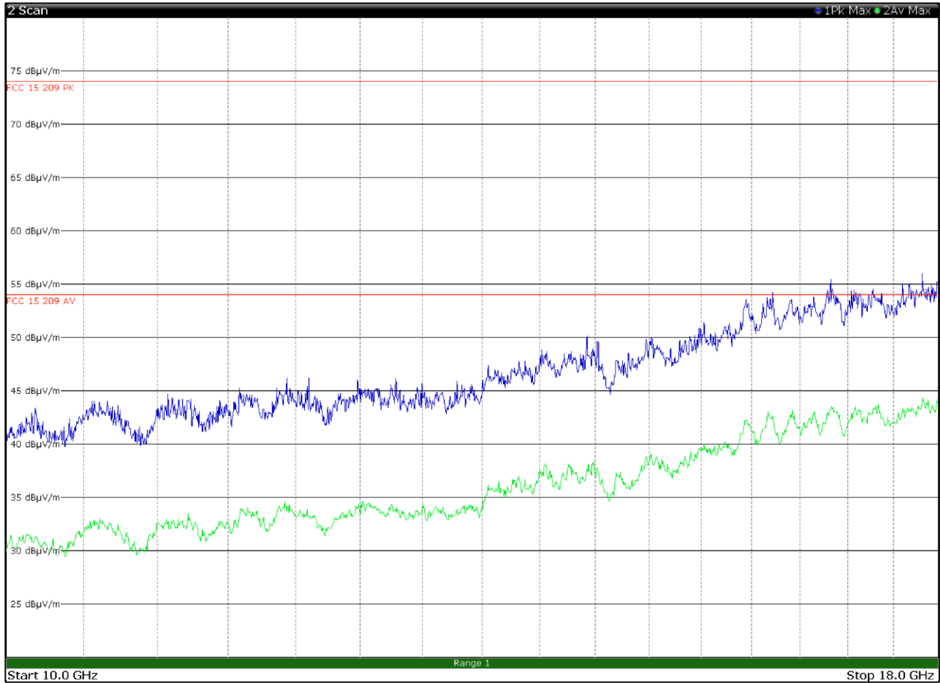
Figure 8.6-19: Radiated spurious emissions 10 to 18 GHz, High channel with antenna in horizontal polarization
