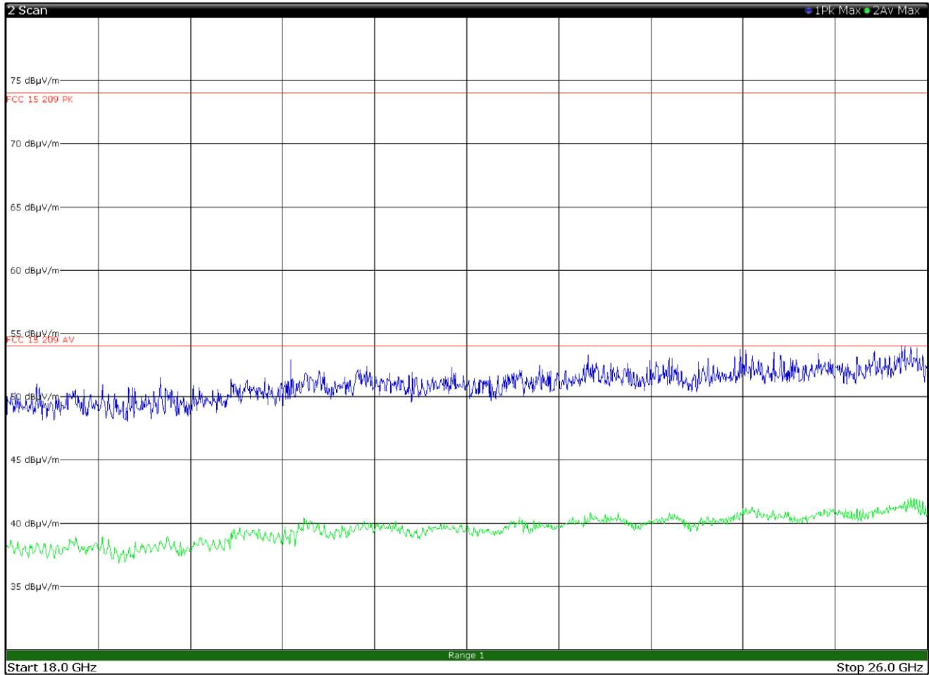
Figure 8.6-25: Radiated spurious emissions 18 to 26 GHz, High channel with antenna in horizontal polarization
