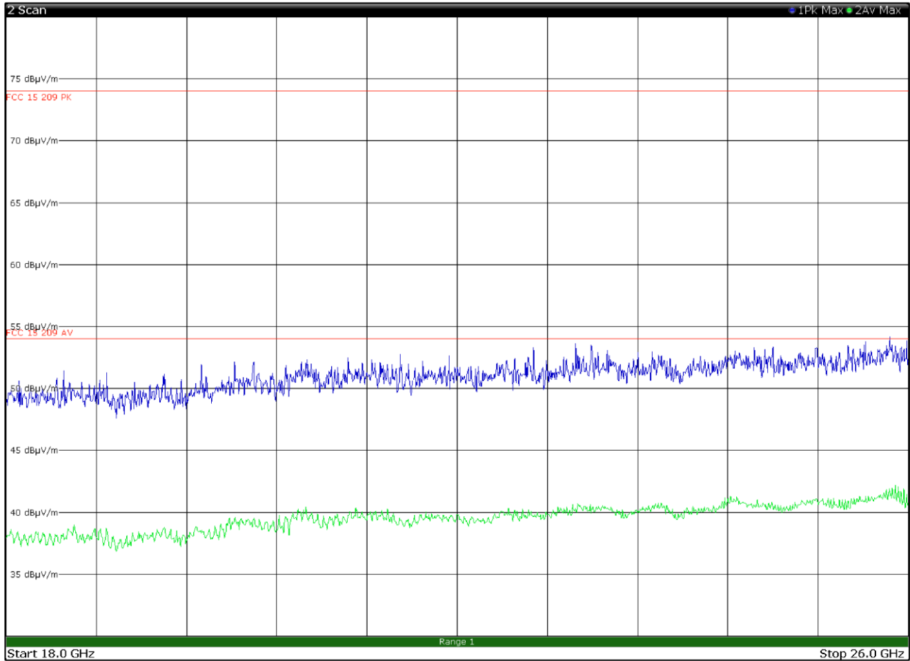
Figure 8.6-24: Radiated spurious emissions 18 to 26 GHz, Mid channel with antenna in vertical polarization
