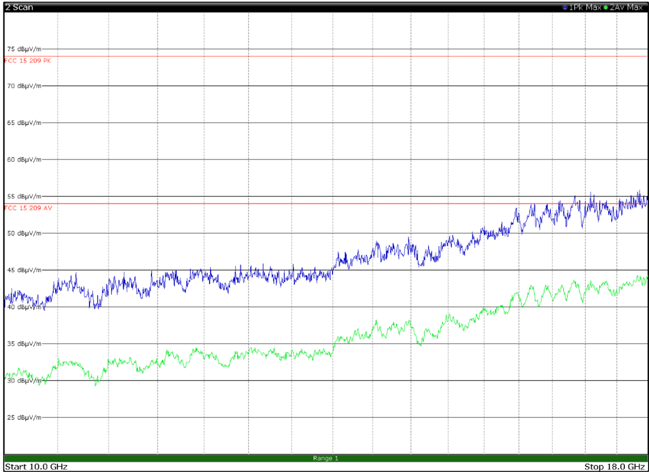
Figure 8.6-18: Radiated spurious emissions 10 to 18 GHz, Mid channel with antenna in vertical polarization
