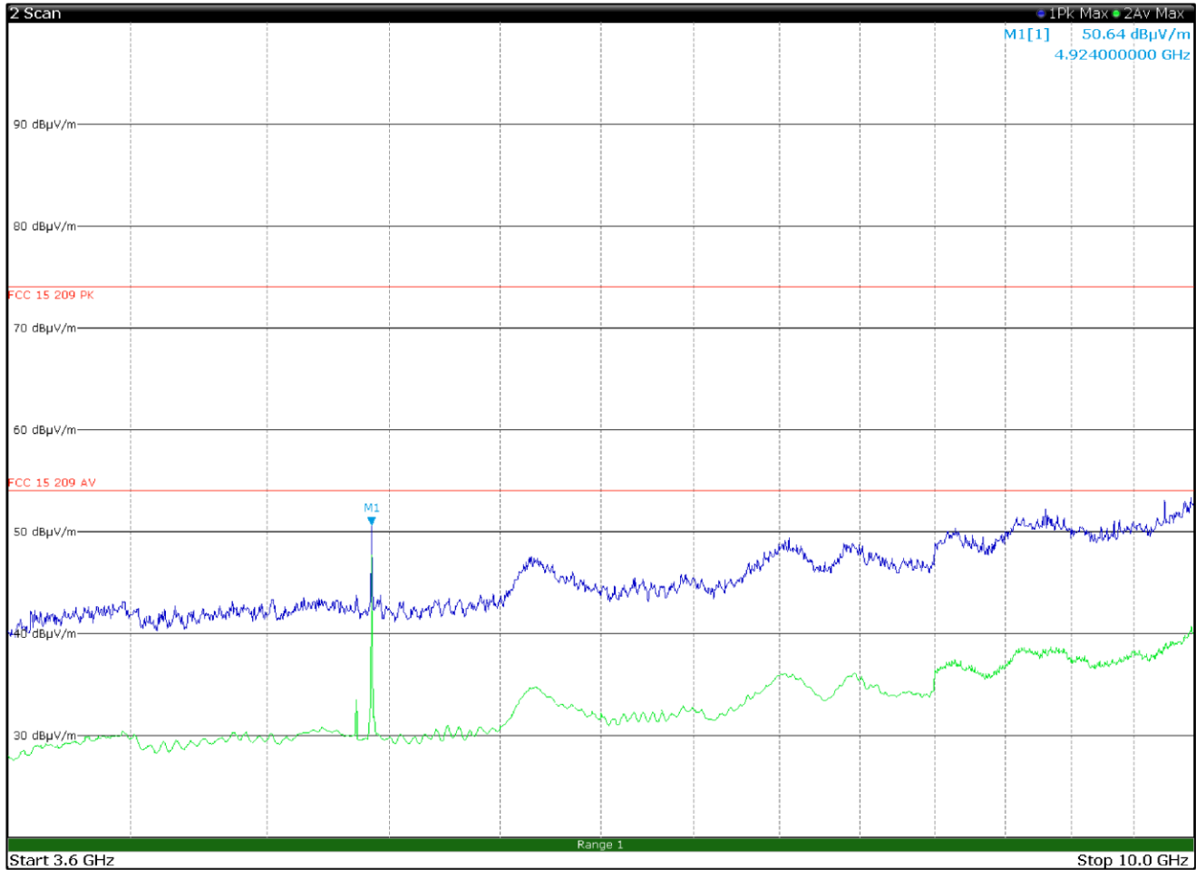
Figure 8.6-13: Radiated spurious emissions 3.6 to 10 GHz, High channel with antenna in horizontal polarization
