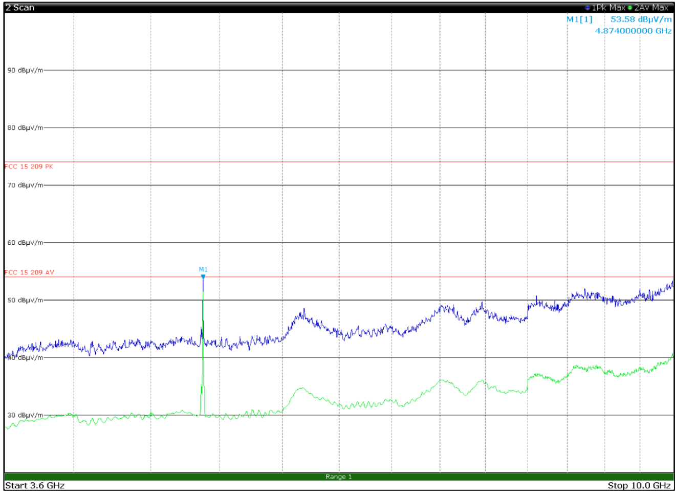
Figure 8.6-12: Radiated spurious emissions 3.6 to 10 GHz, Mid channel with antenna in vertical polarization
