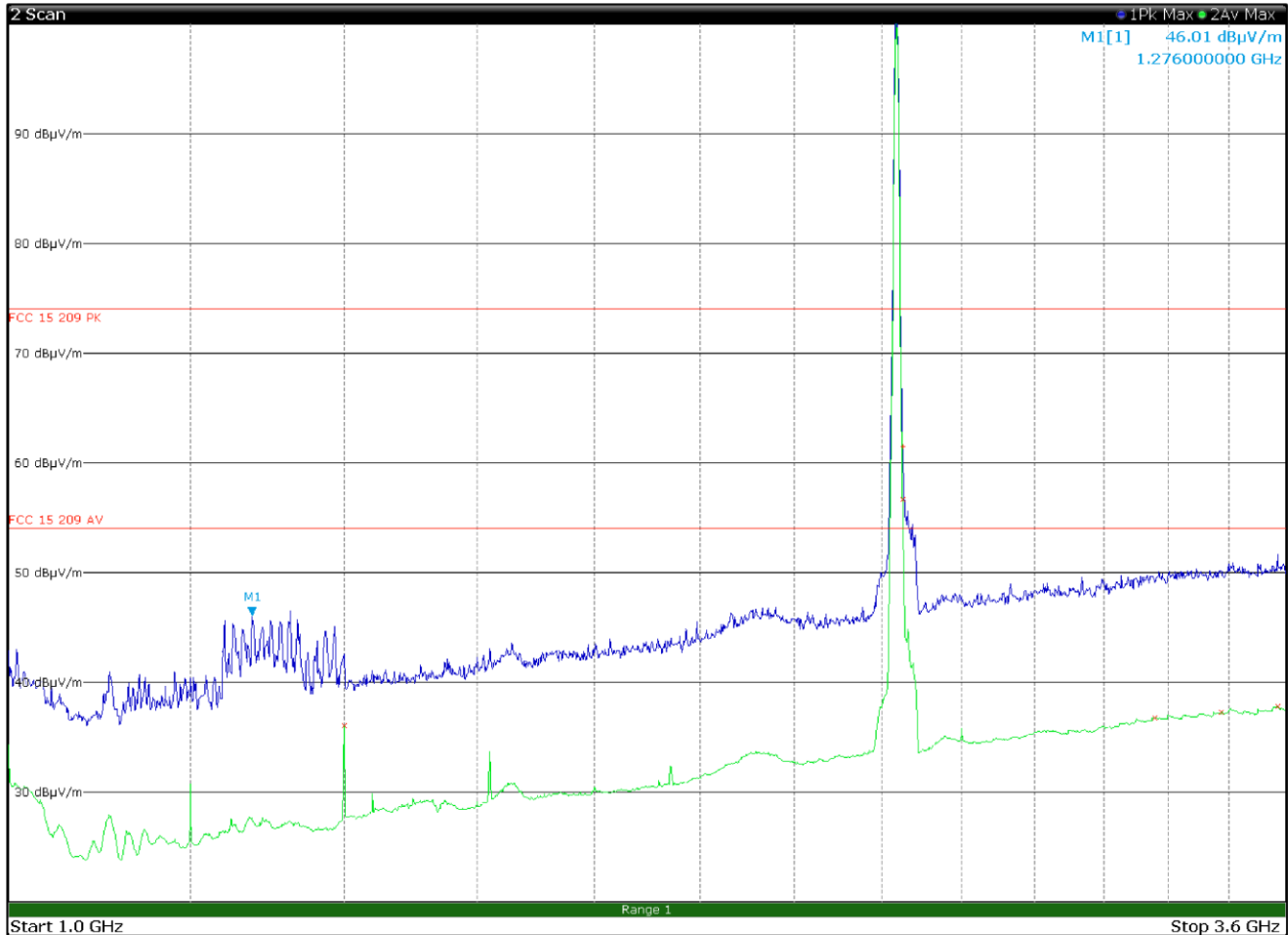
Figure 8.6-6: Radiated spurious emissions 1 to 3.6 GHz, Mid channel with antenna in vertical polarization
