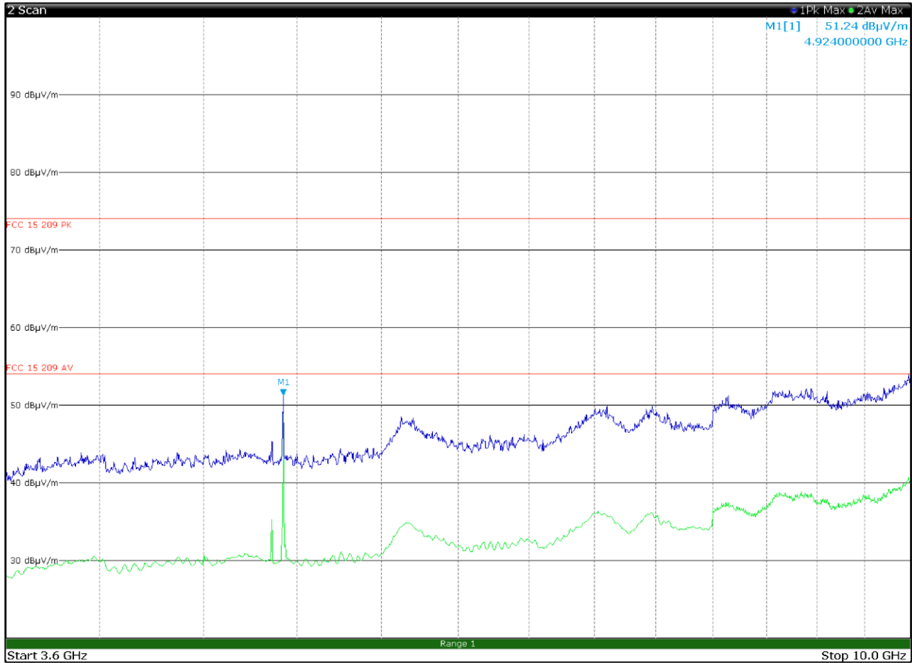
Figure 8.6-14: Radiated spurious emissions 3.6 to 10 GHz, High channel with antenna in vertical polarization
