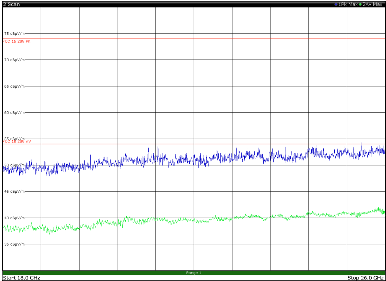
Figure 8.6-23: Radiated spurious emissions 18 to 26 GHz, Mid channel with antenna in horizontal polarization
