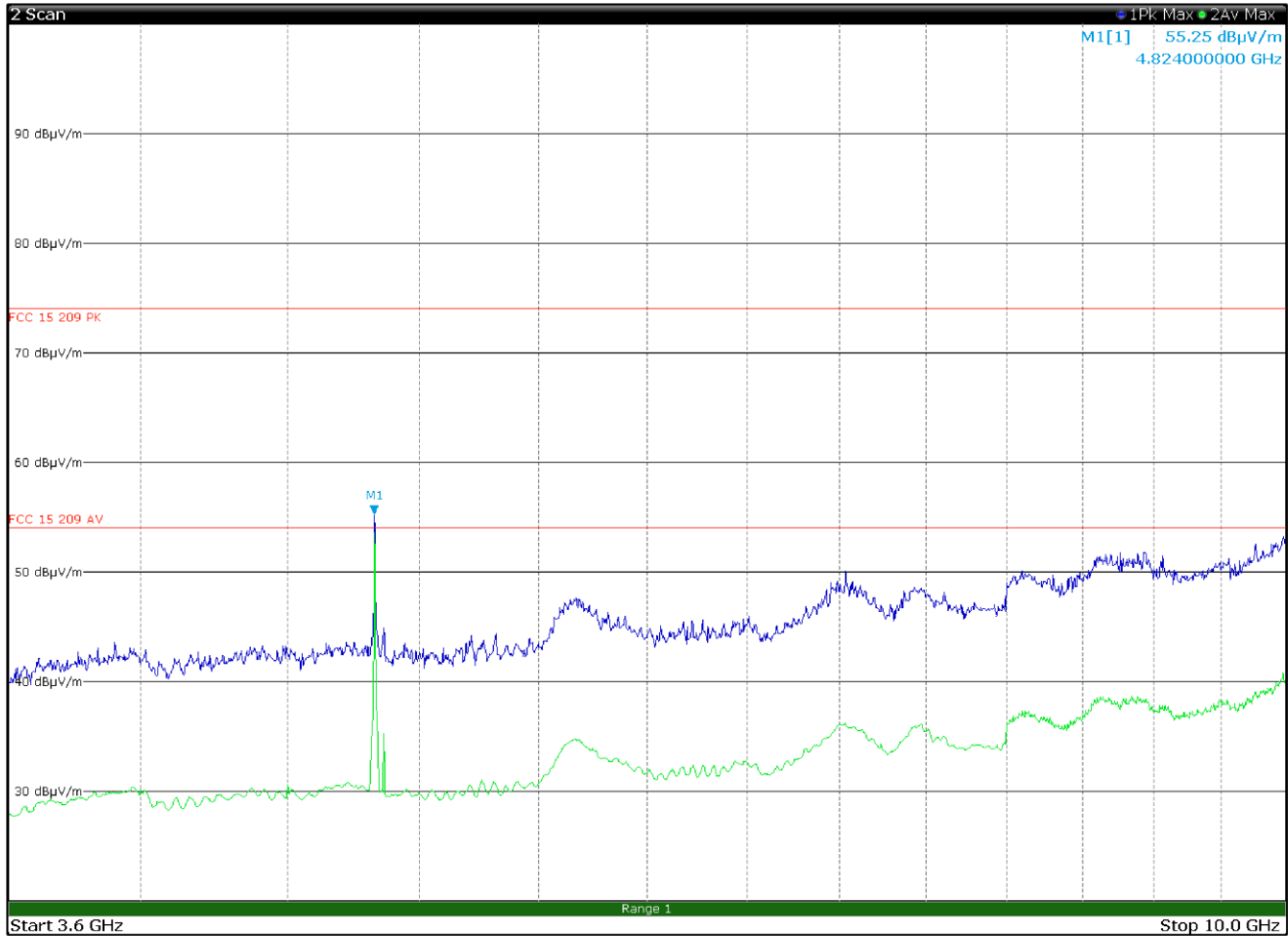
Figure 8.6-10: Radiated spurious emissions 3.6 to 10 GHz, Low channel with antenna in vertical polarization
