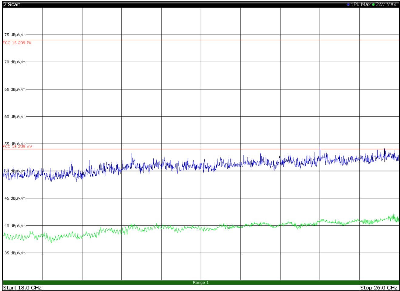
Figure 8.6-26: Radiated spurious emissions 18 to 26 GHz, High channel with antenna in vertical polarization
