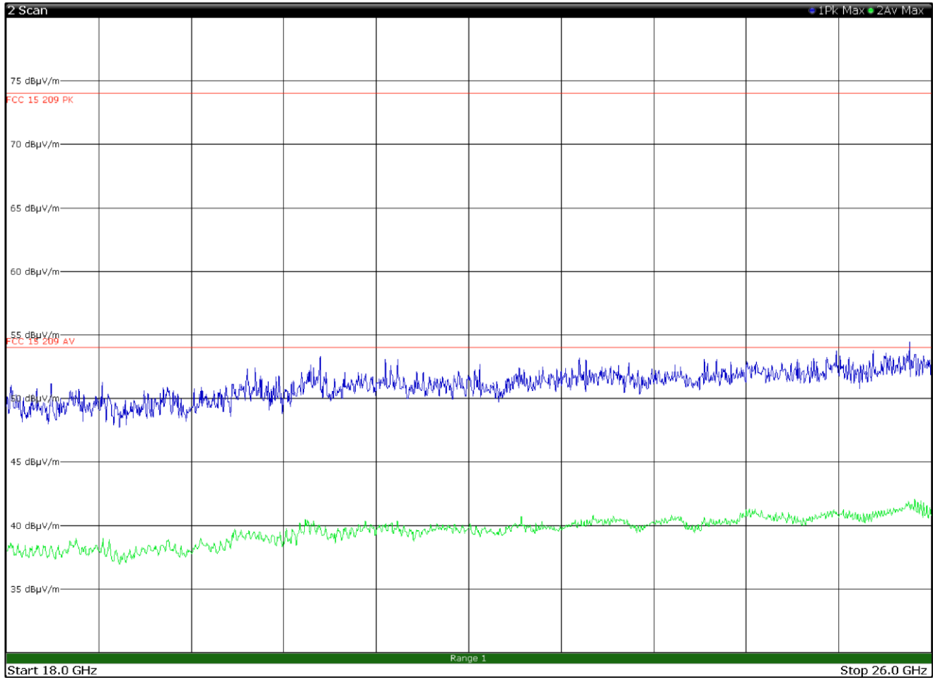
Figure 8.6-21: Radiated spurious emissions 18 to 26 GHz, Low channel with antenna in horizontal polarization
