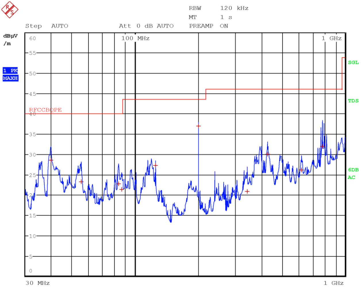
Figure 8.6-2: Radiated spurious emissions 30 to 1000 MHz, Mid channel with antenna in vertical polarization
