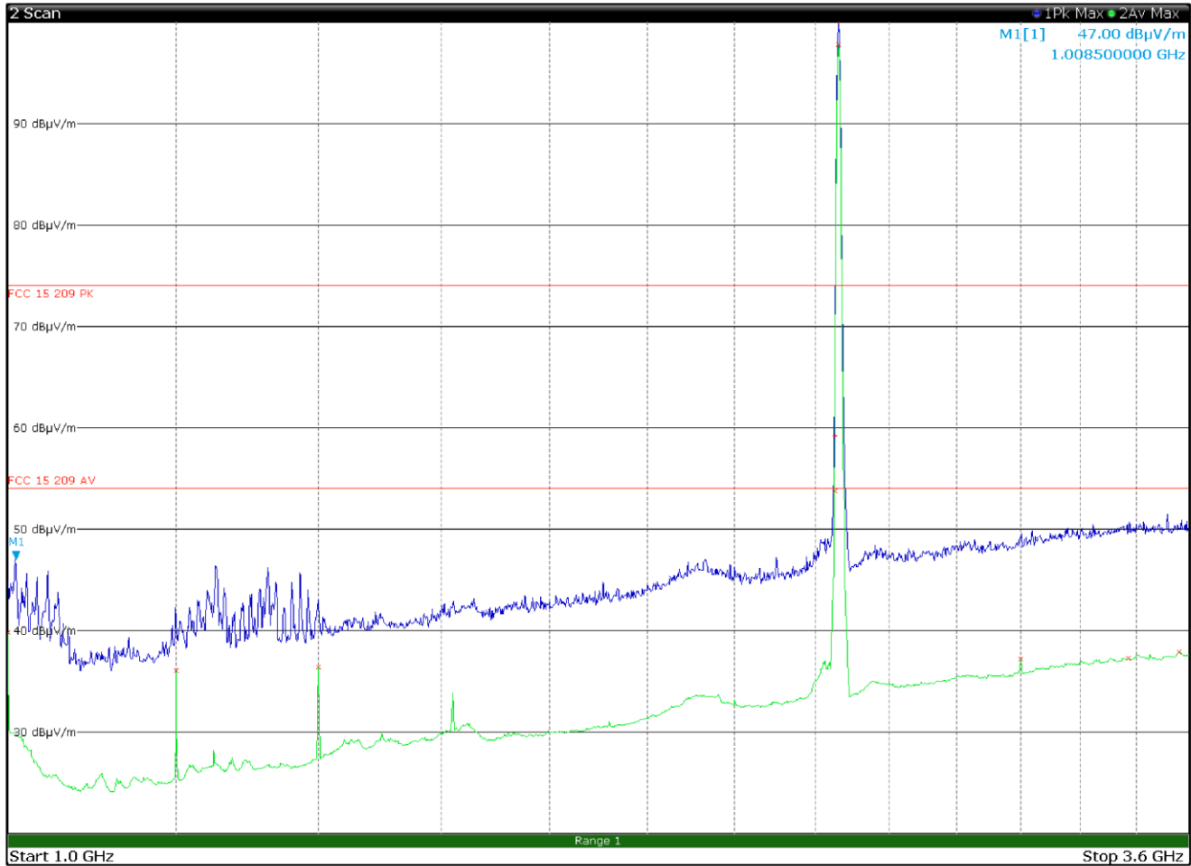
Figure 8.6-7: Radiated spurious emissions 1 to 3.6 GHz, High channel with antenna in horizontal polarization
