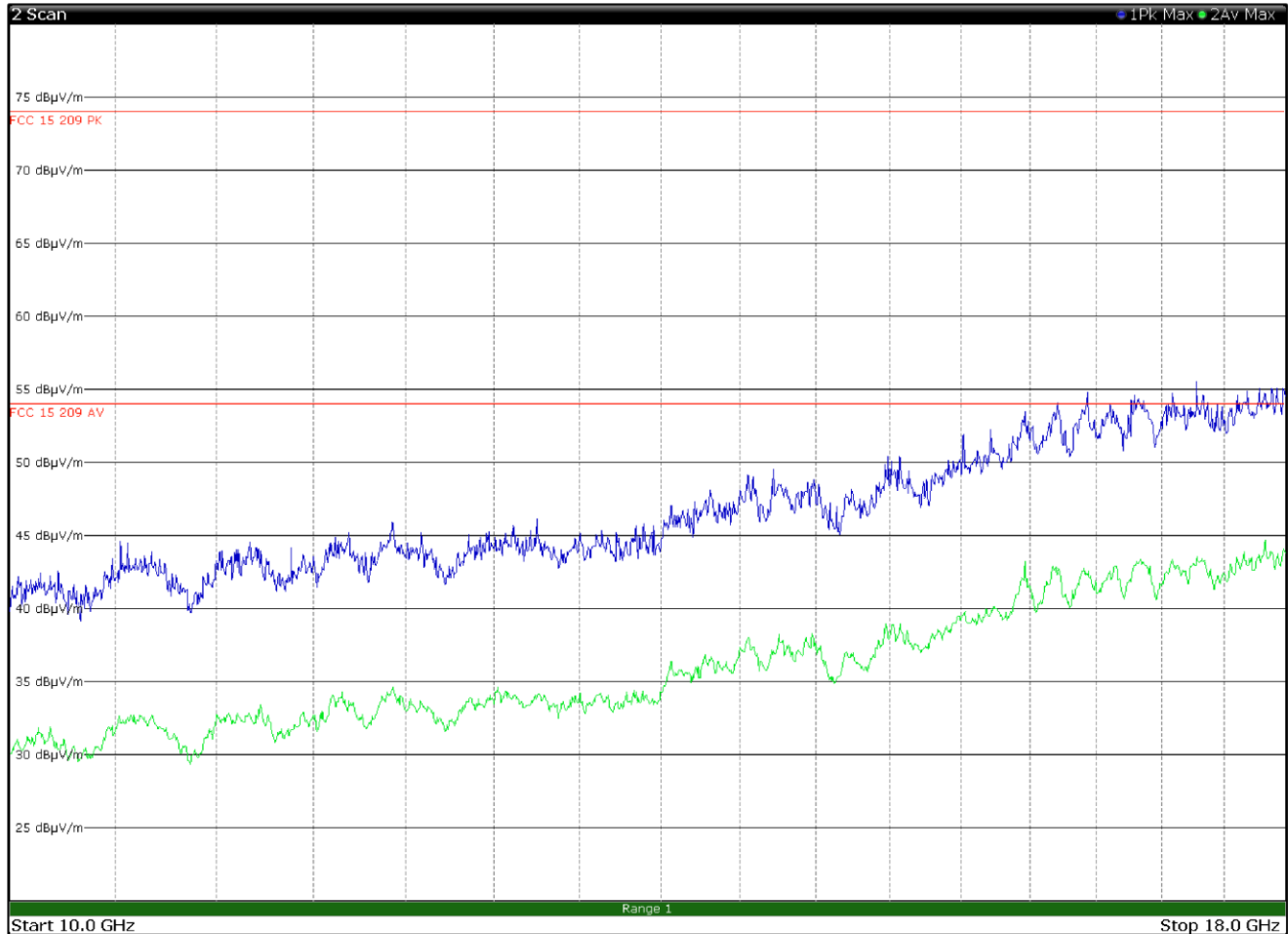
Figure 8.6-16: Radiated spurious emissions 10 to 18 GHz, Low channel with antenna in vertical polarization
