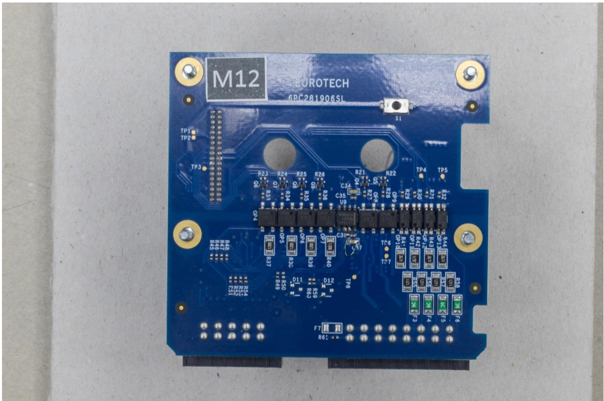
Figure 5 – IO BOTTOM
