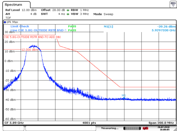
Figure 8.4-12: Upper band edge, Tx on ch 165, 802.11n HT20
