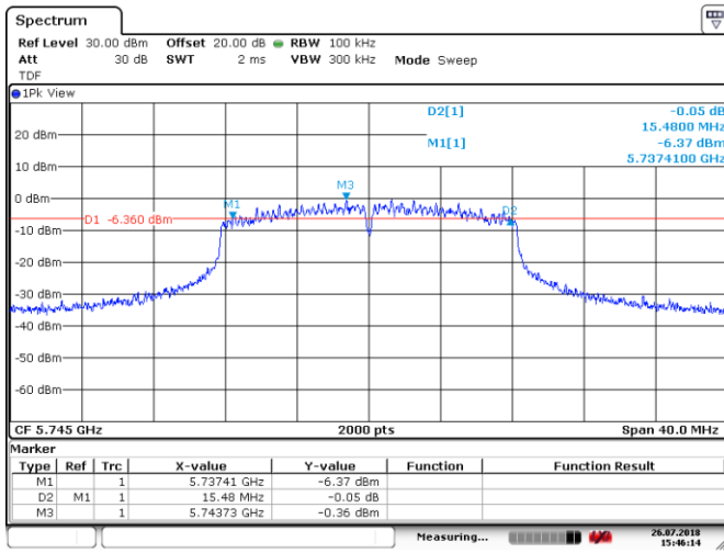
Figure 8.1-4: 6 dB bandwidth on 802.11a, sample plot
