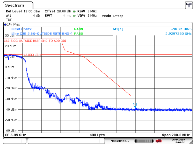
Figure 8.4-14: Upper band edge, Tx on ch 159, 802.11n HT40
