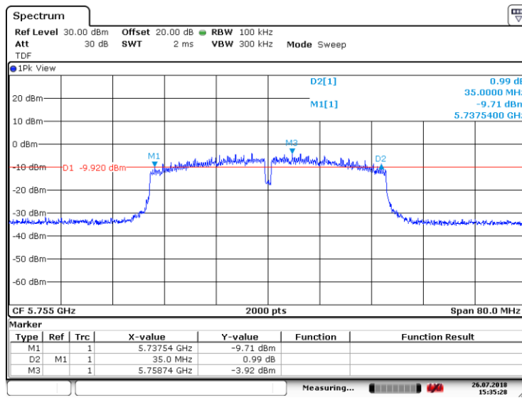
Figure 8.1-6: 6 dB bandwidth on 802.11n HT40, sample plot
