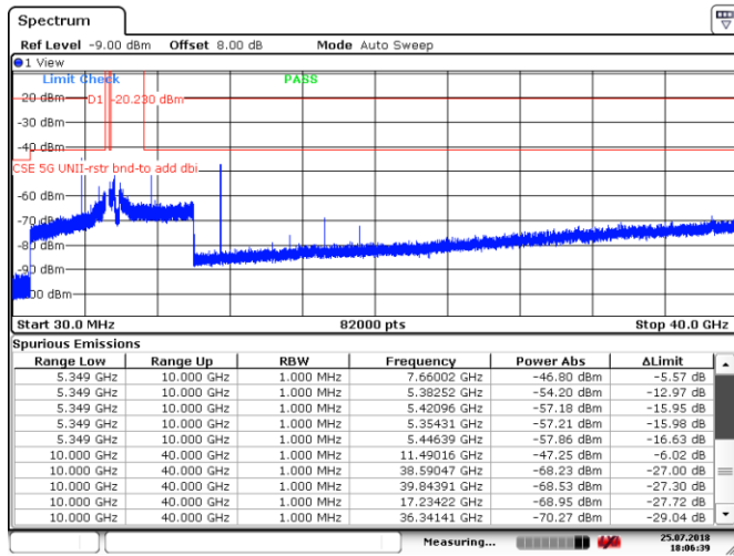
Figure 8.4-19: Spurious emissions within restricted bands, Tx on ch 149, 802.11n HT20
