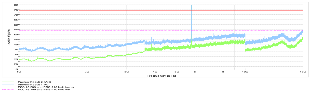
Figure 8.4-25: Cabinet Radiated spurious emission 1 to 18 GHz Tx on low channel
