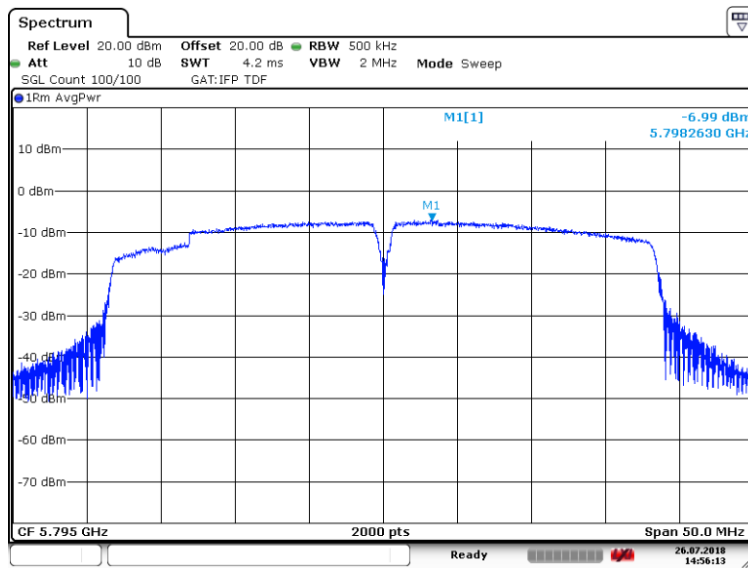
Figure 8.3-3: PSD on 802.11n HT40, Sample plot
