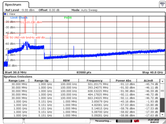
Figure 8.4-20: Spurious emissions within restricted bands, Tx on ch 157, 802.11n HT20
