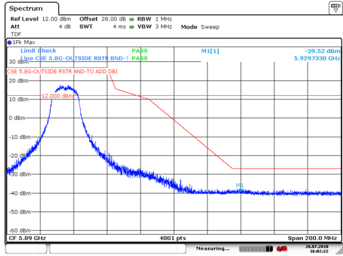
Figure 8.4-10: Upper band edge, Tx on ch 165, 802.11a
