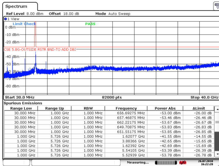
Figure 8.4-6: Spurious emissions outside restricted bands, Tx on ch 165, 802.11n HT20
