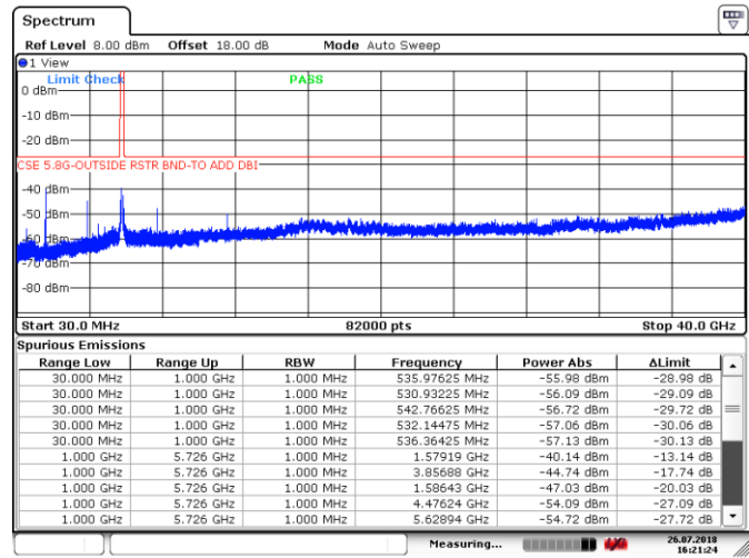
Figure 8.4-5: Spurious emissions outside restricted bands, Tx on ch 157, 802.11n HT20
