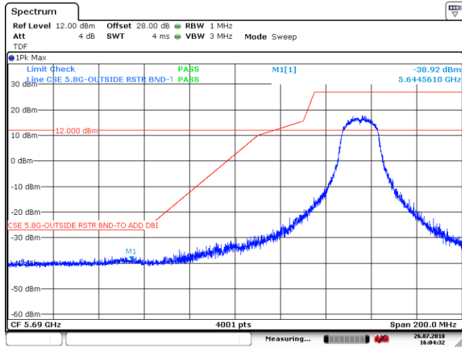
Figure 8.4-9: Lower band edge, Tx on ch 149, 802.11a
