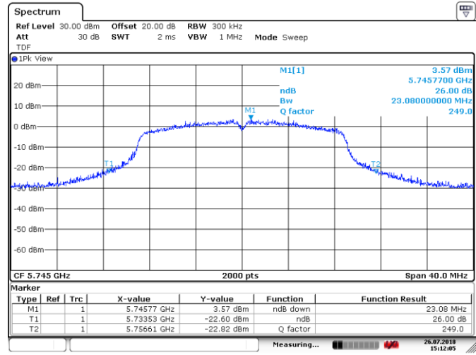
Figure 8.1-2: 26 dB bandwidth on 802.11n HT20, sample plot
