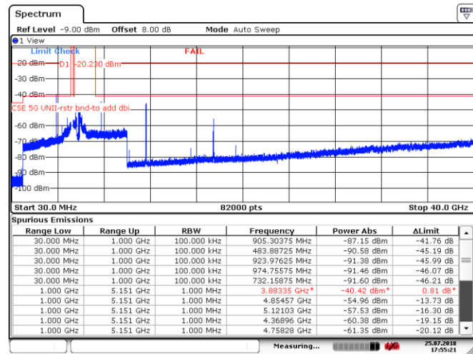
Figure 8.4-17: Spurious emissions within restricted bands, Tx on ch 165, 802.11a, Peak measurement
