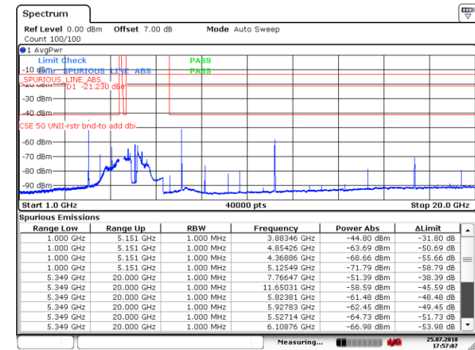
Figure 8.4-18: Spurious emissions within restricted bands, Tx on ch 165, 802.11a, Average measurement
