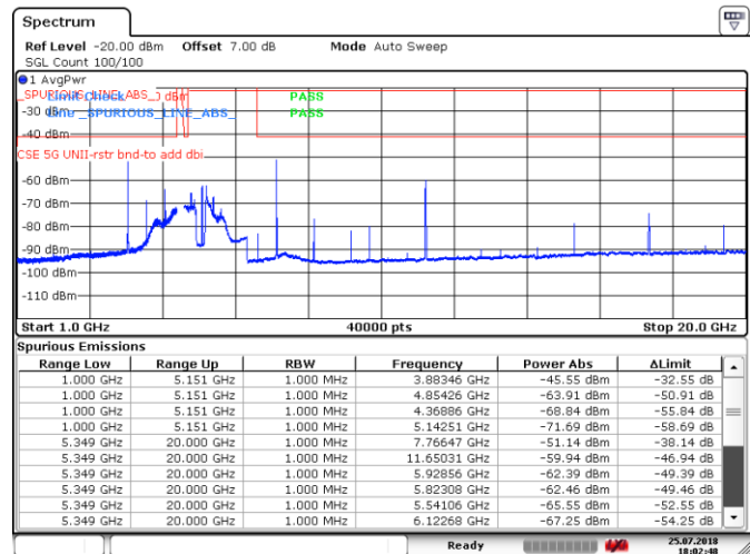
Figure 8.4-22: Spurious emissions within restricted bands, Tx on ch 165, 802.11n HT20, Average measurement
