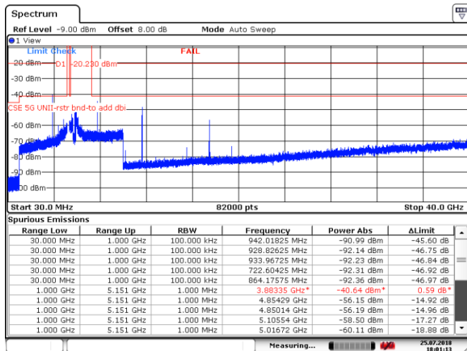
Figure 8.4-21: Spurious emissions within restricted bands, Tx on ch 165, 802.11n HT20, Peak measurement
