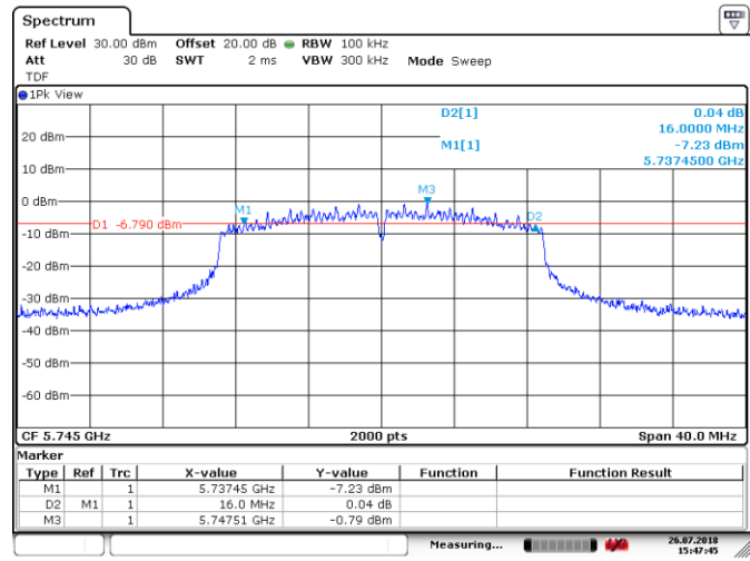
Figure 8.1-5: 6 dB bandwidth on 802.11n HT20, sample plot
