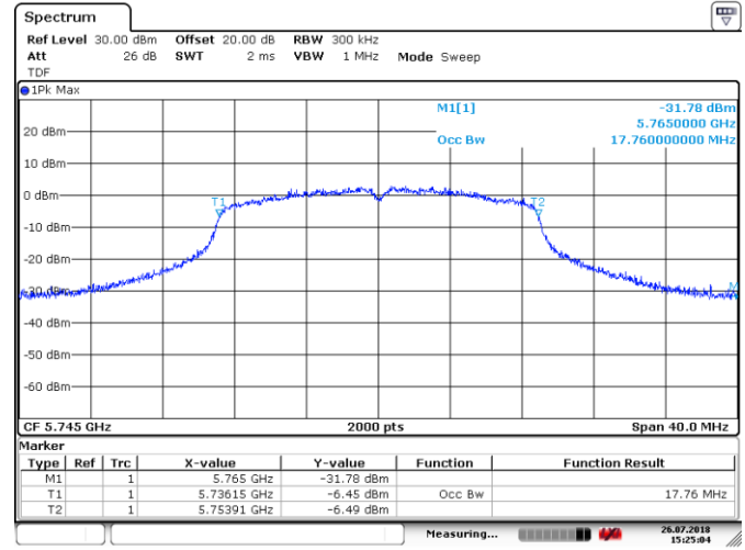
Figure 8.2-2: 99 % bandwidth on 802.11n HT20, sample plot
