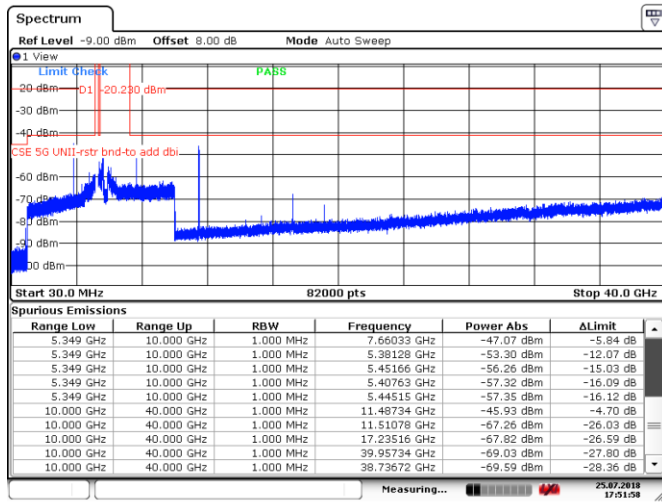
Figure 8.4-15: Spurious emissions within restricted bands, Tx on ch 149, 802.11a
