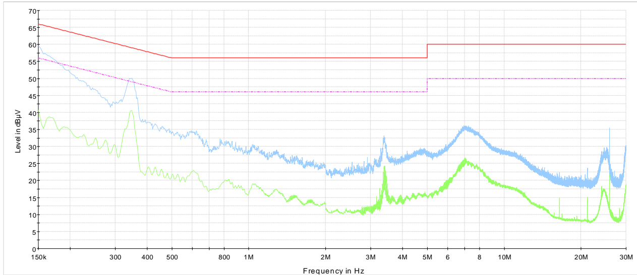
Preview Result 2-AVG Preview Result 1-PK+ CISPR 32 Limit - Class B, Mains (Quasi-Peak) CISPR 32 Limit - Class B, Mains (Average)
