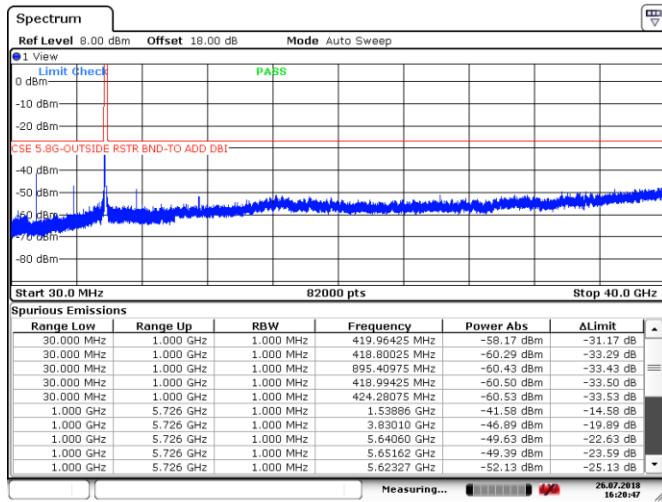
Figure 8.4-4: Spurious emissions outside restricted bands, Tx on ch 149, 802.11n HT20
