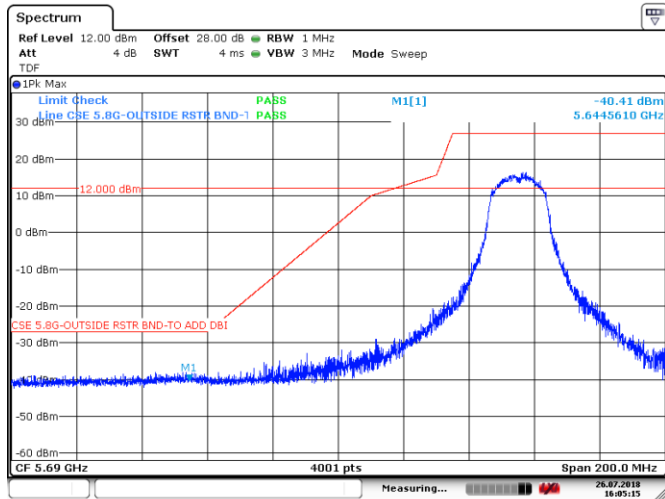
Figure 8.4-11: Lower band edge, Tx on ch 149, 802.11n HT20
