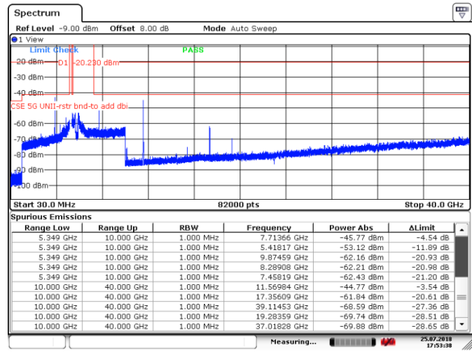
Figure 8.4-16: Spurious emissions within restricted bands, Tx on ch 157, 802.11a
