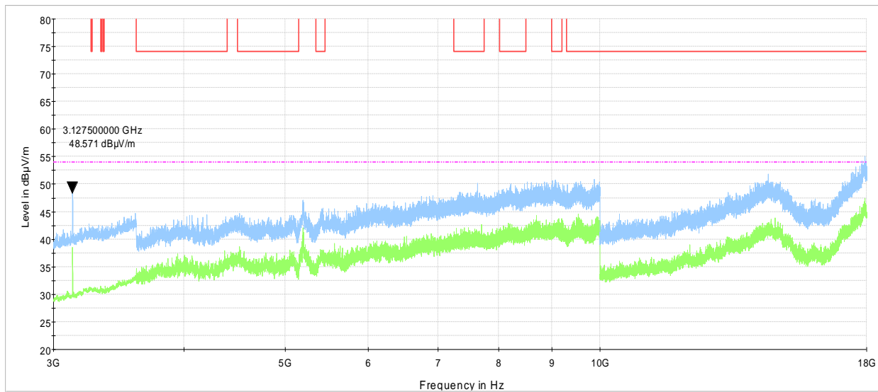
Figure 8.1-9: Radiated spurious emissions, LTE Tx at 782 MHz, WiFi Tx at 2412 MHz
