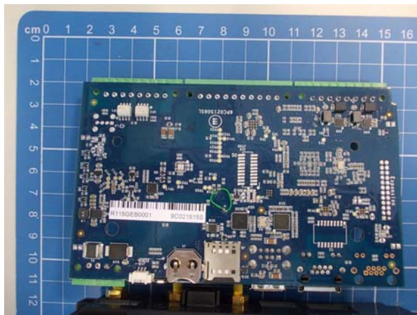
Main board bottom side
