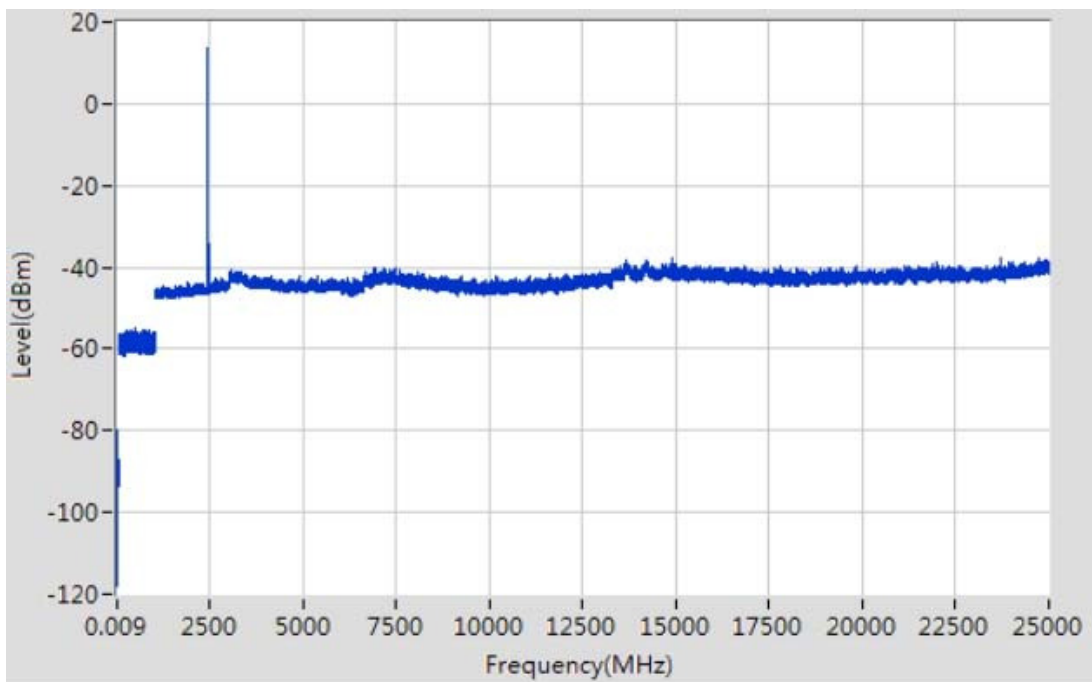
Middle CHANNEL, SPURIOUS, 9 kHz ~ 25 GHz
