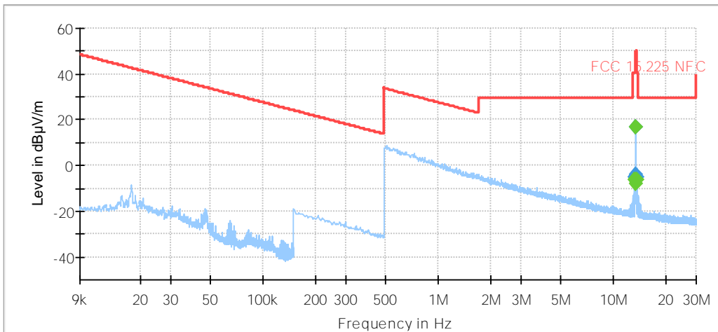
◆ Preview Result 1-PK+ Final_Result PK+ ◆ FCC 15.225 NFC Final_Result QPK
