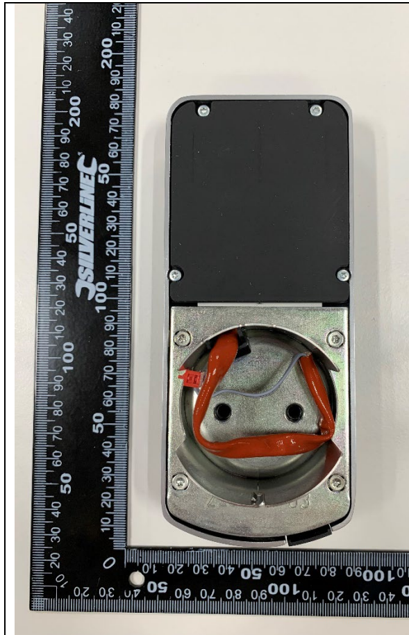
Photo 7: External part bottom view.
