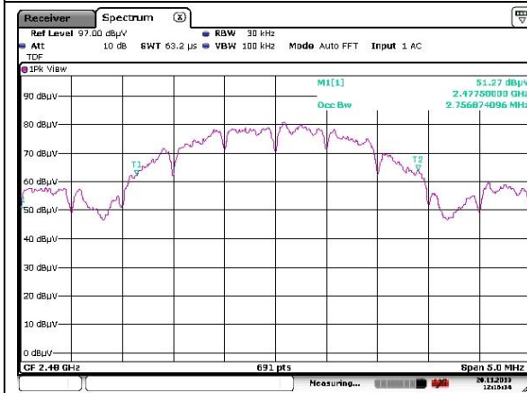
Ch 26: 99% emission bandwidth: 2.76 MHz
