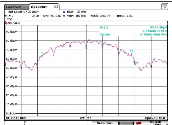
Ch 19: 99% emission bandwidth: 2.76 MHz
