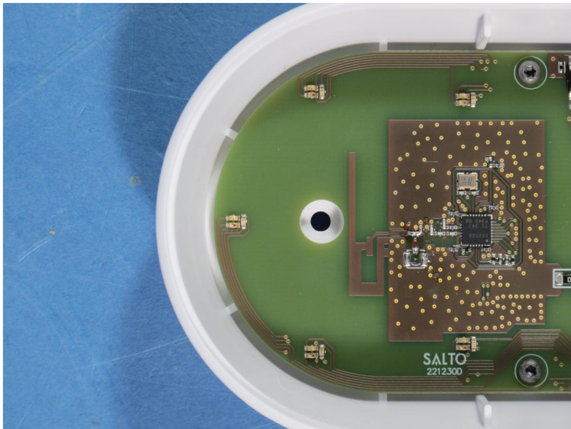
Photograph 3: View on Zigbee module plus antenna
