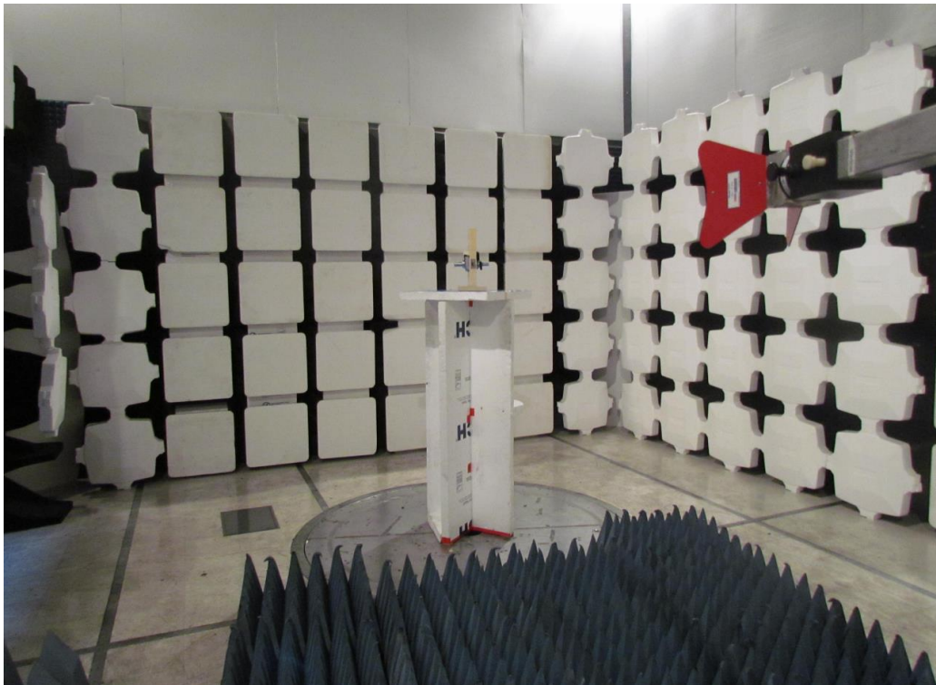
Radiated Emissions above 1GHz
