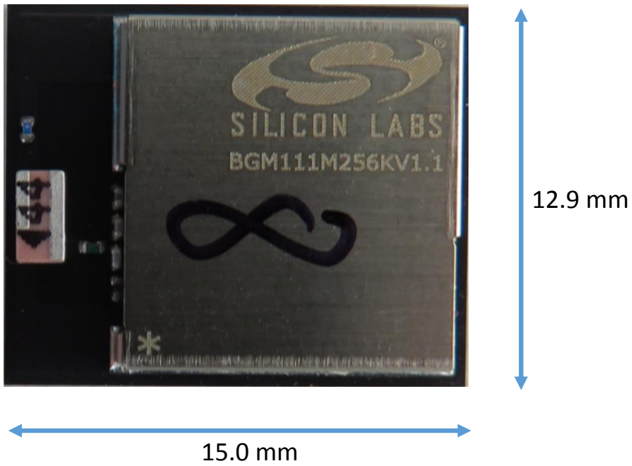
Figure 1: BGM111 External Photo, top view
