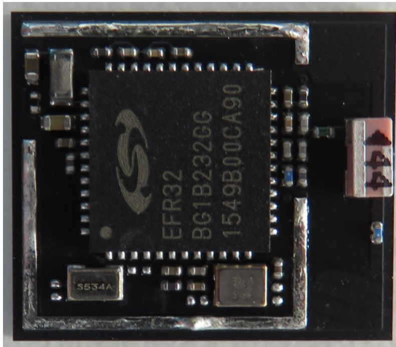
Figure 2: BGM111 Internal Photo
