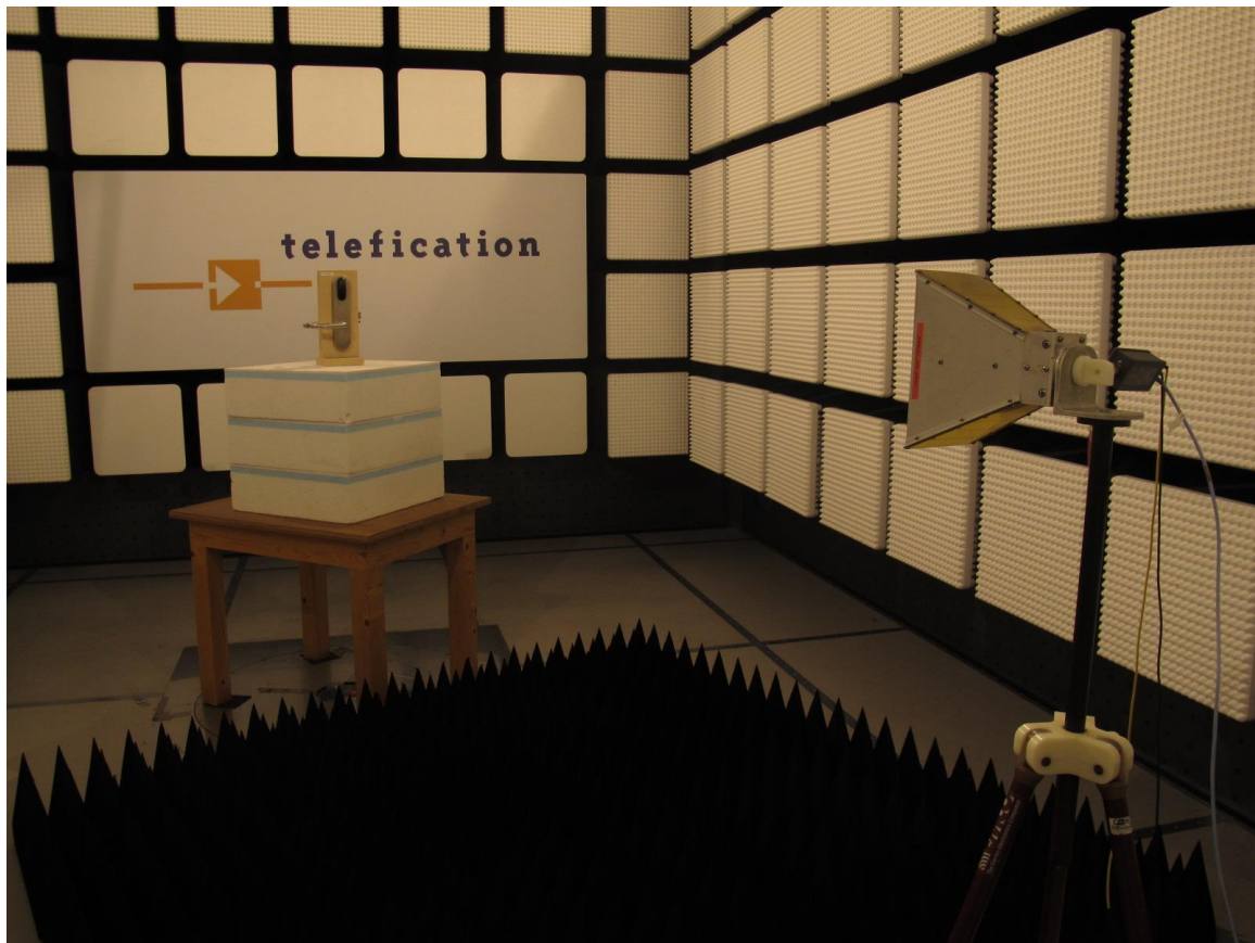
Photograph 2: Radiated emissions test set up, 1 – 18 GHz
