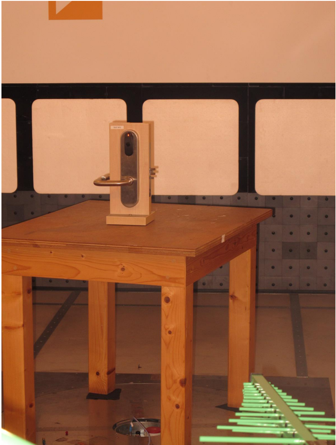
Photograph 4: Test setup radiated emissions 0.03 - 1 GHz
