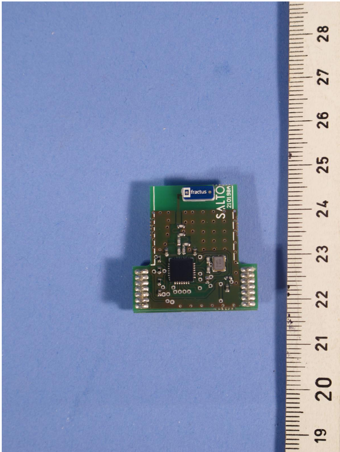
Photograph 4: Top view on radio module
