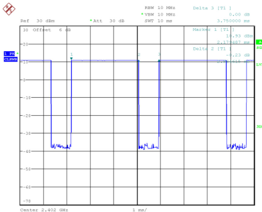
Time-domain plot for Bluetooth transmission signal
