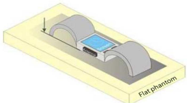
Fig-4.2 Illustration for Wireless Watch Setup
