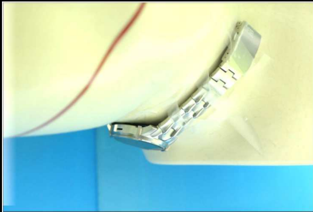
Neck Region of EUT Tested at 0 mm(Sample D2)
