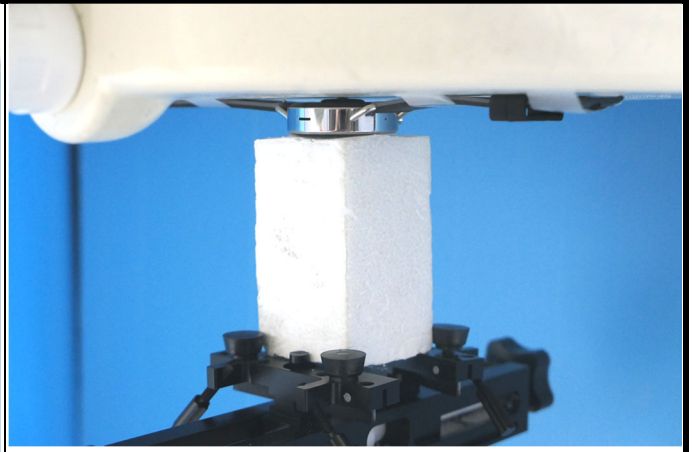
Rear Face of EUT Tested at 0 mm_DW13S1(Plastic)
