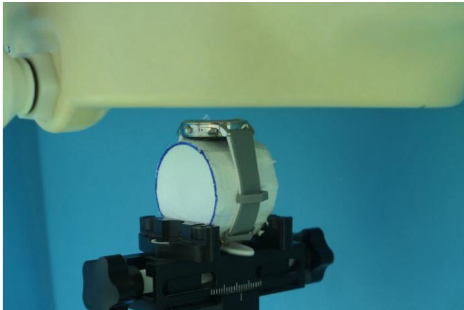
Fig-4.5 Front Face of EUT with 10 mm Gap (Sample A)
