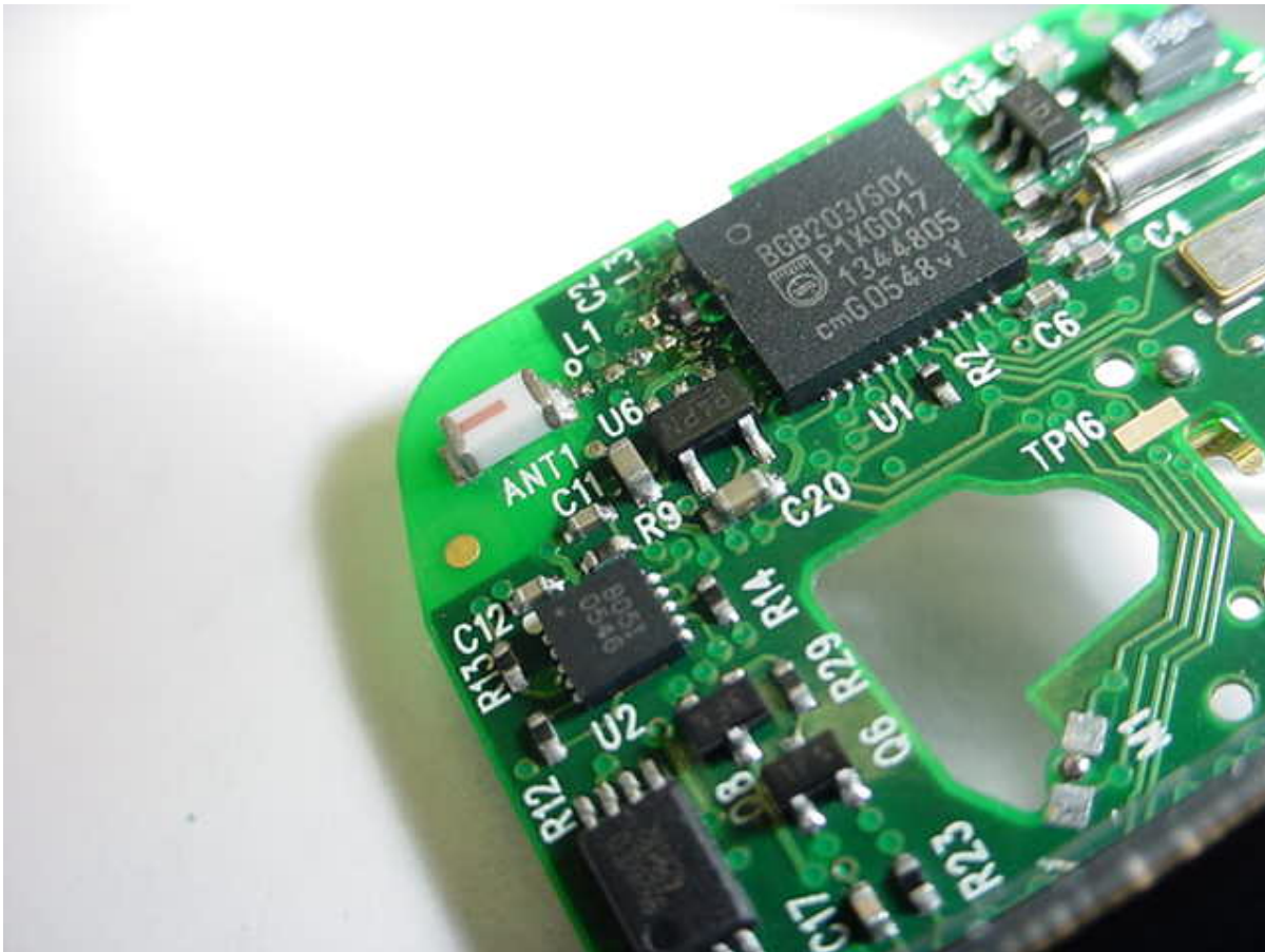
Photo Five – Internal View of Chip Antenna
