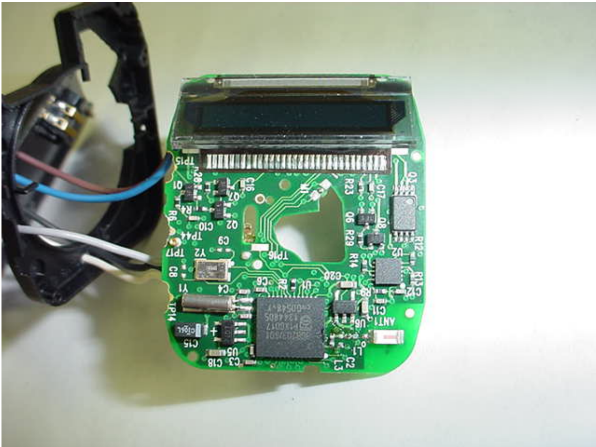
Photo Three – Internal Component Side with RF Circuitry
