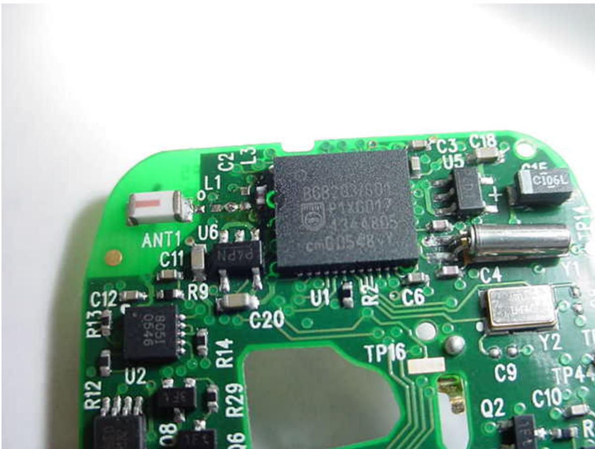
Photo Four – Internal RF Section with Bluetooth Chip
