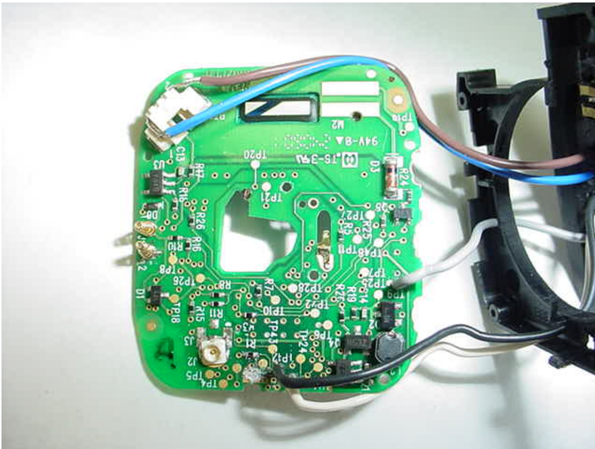
Photo Two – Internal Non RF Component Side, with Test Leads
