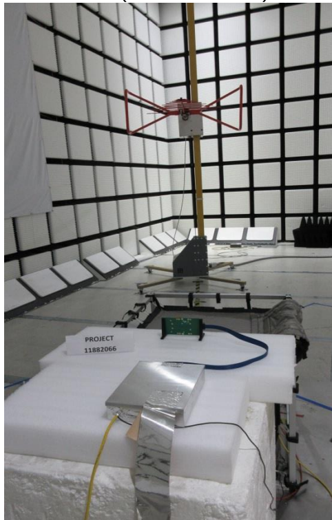
RADIATED BACK PHOTO (BELOW 1 GHz)
