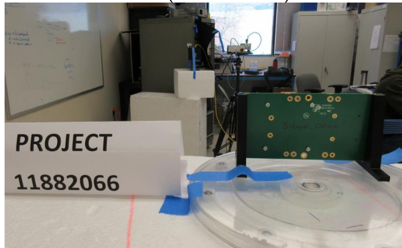
RADIATED BACK PHOTO (FUNDAMENTAL)
