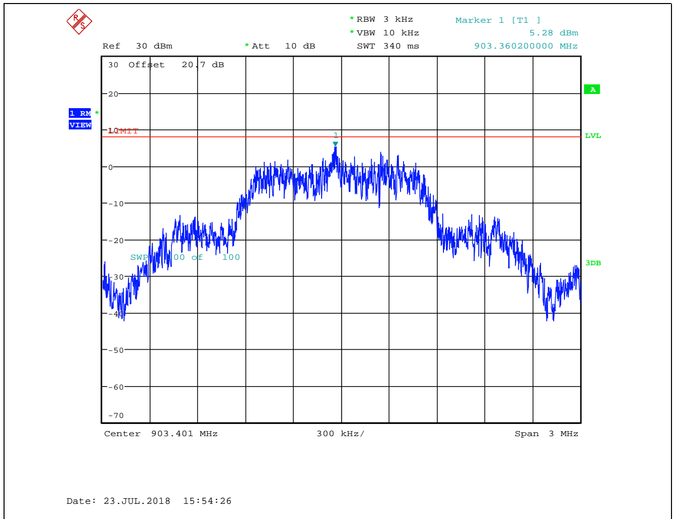
Plot 5.5.4.1. Power Spectral Density, 903.401 MHz, FSK modulation Detector RMS, Video Trace Averaging with 100 Traces, Sweep Points 5000 \geq 2 \times \text{Span/RBW}
