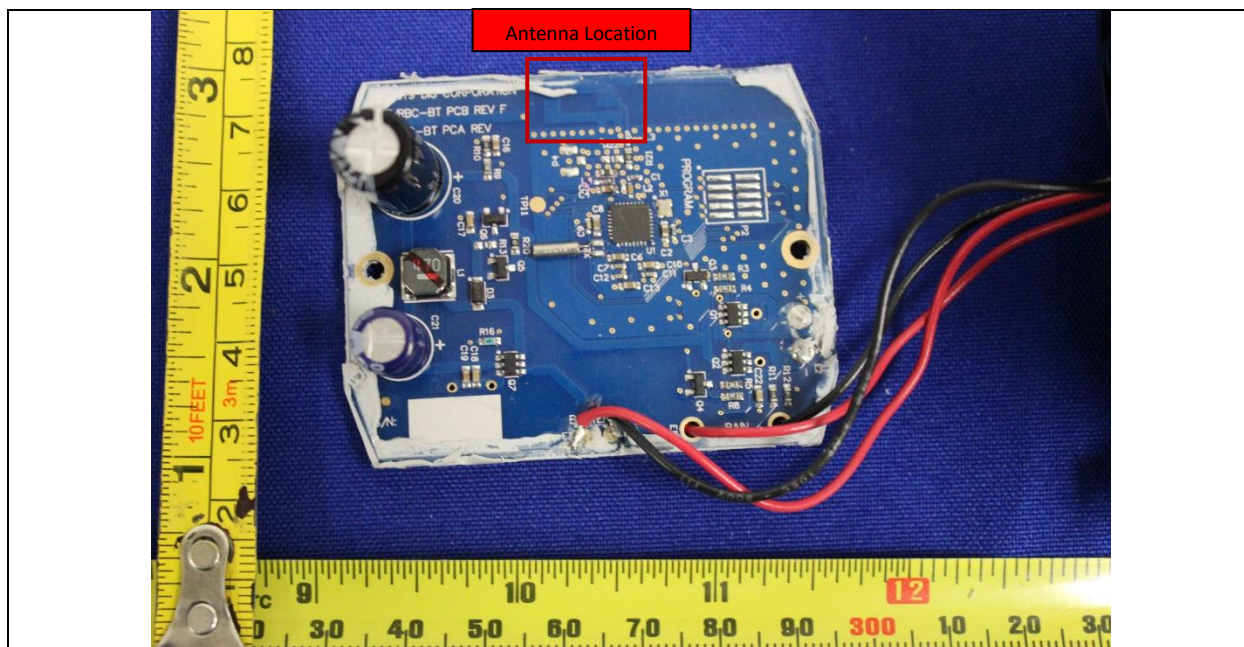
EUT Antenna Top View
