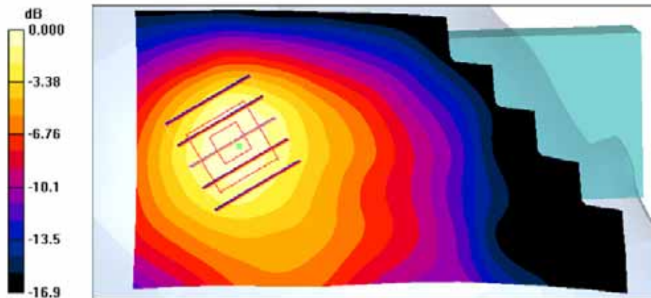
0 dB = 0.080mW/g
