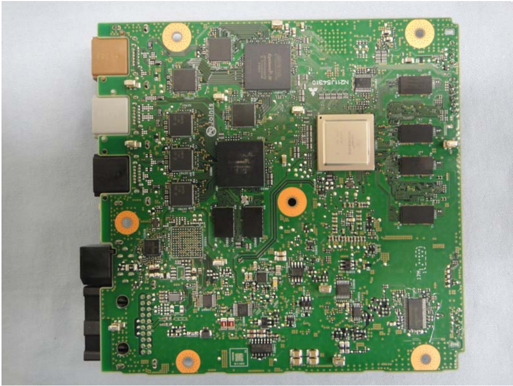
Board Bottom
