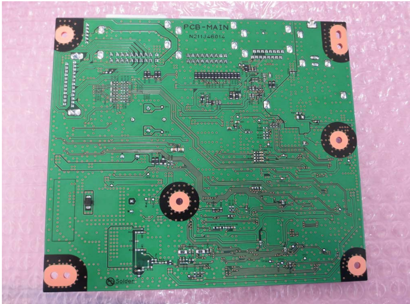
6. PCB-MAIN S-side
