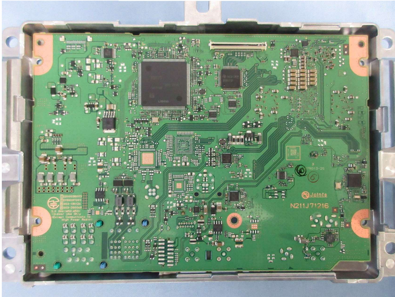
PCB-MAIN S-side
