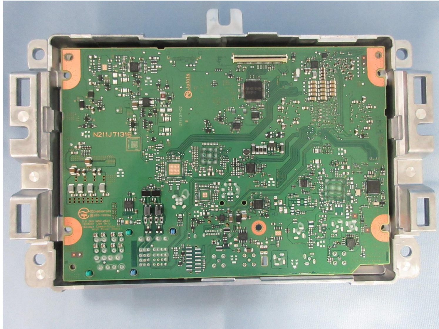
PCB-MAIN S-side
