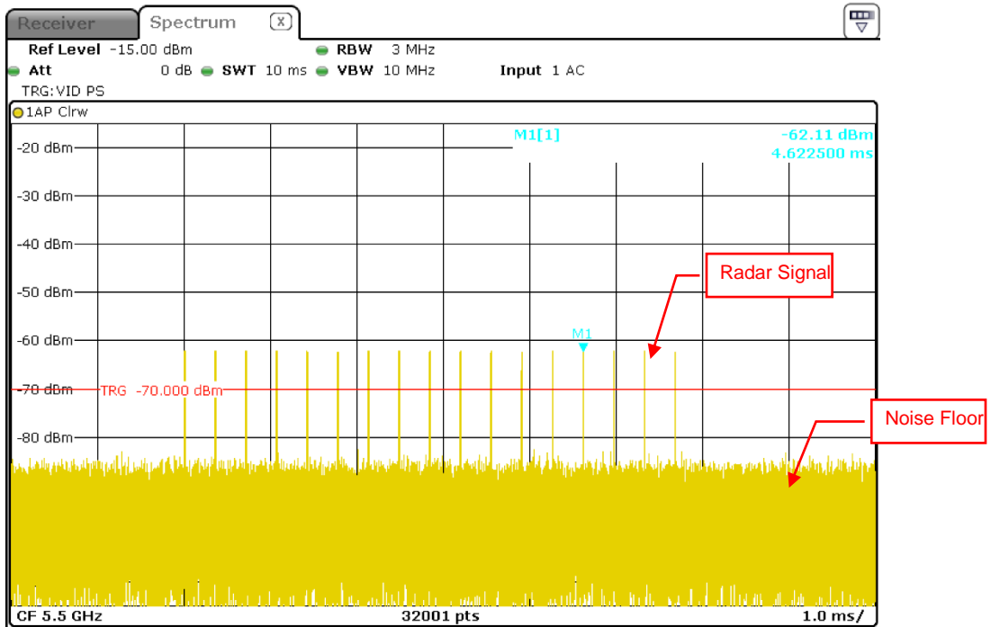
Radar Signal 3
