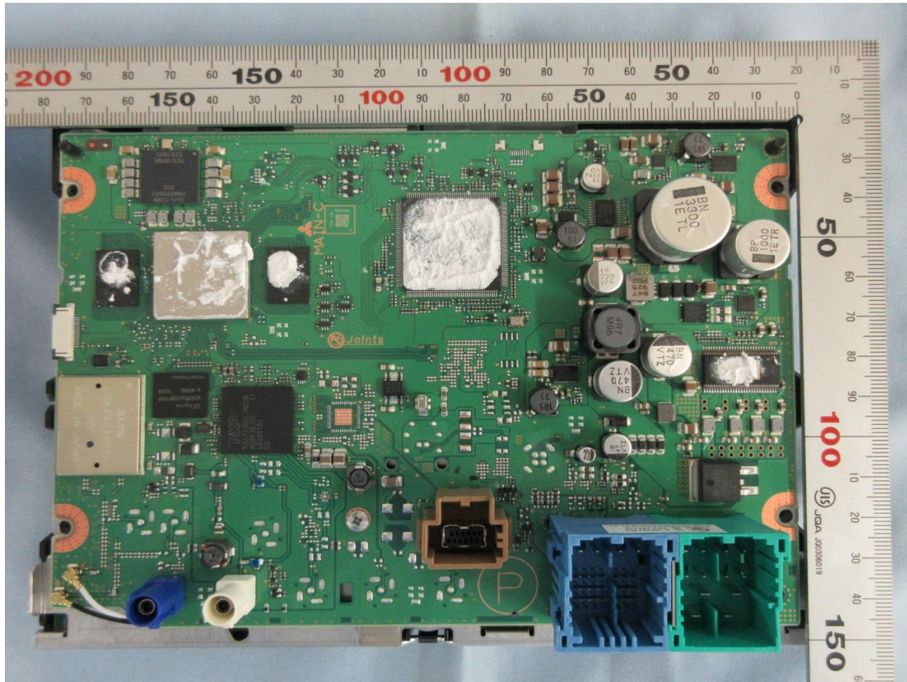
1. PCB-MAIN C-side
