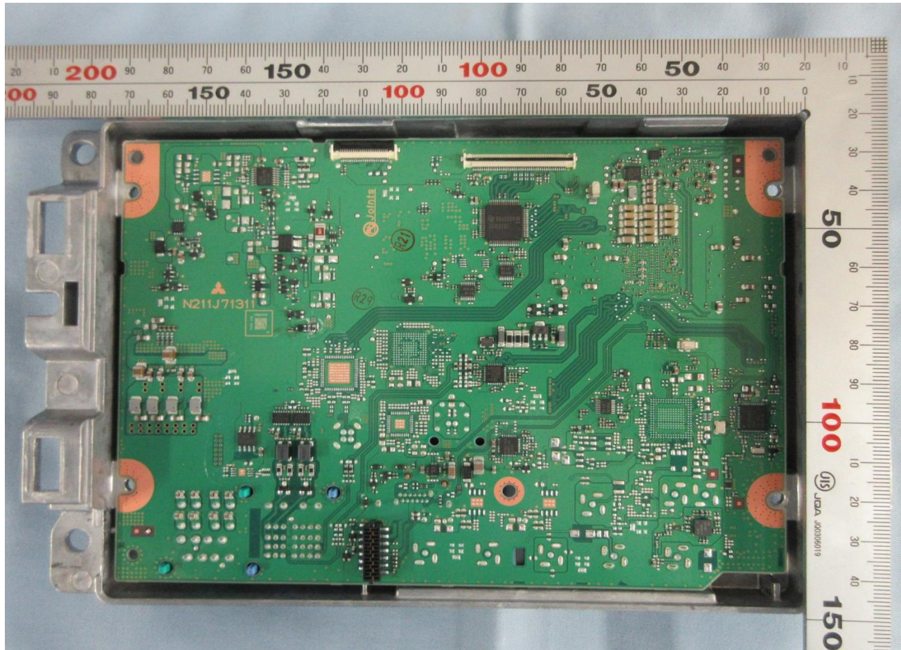
2. PCB-MAIN S-side
