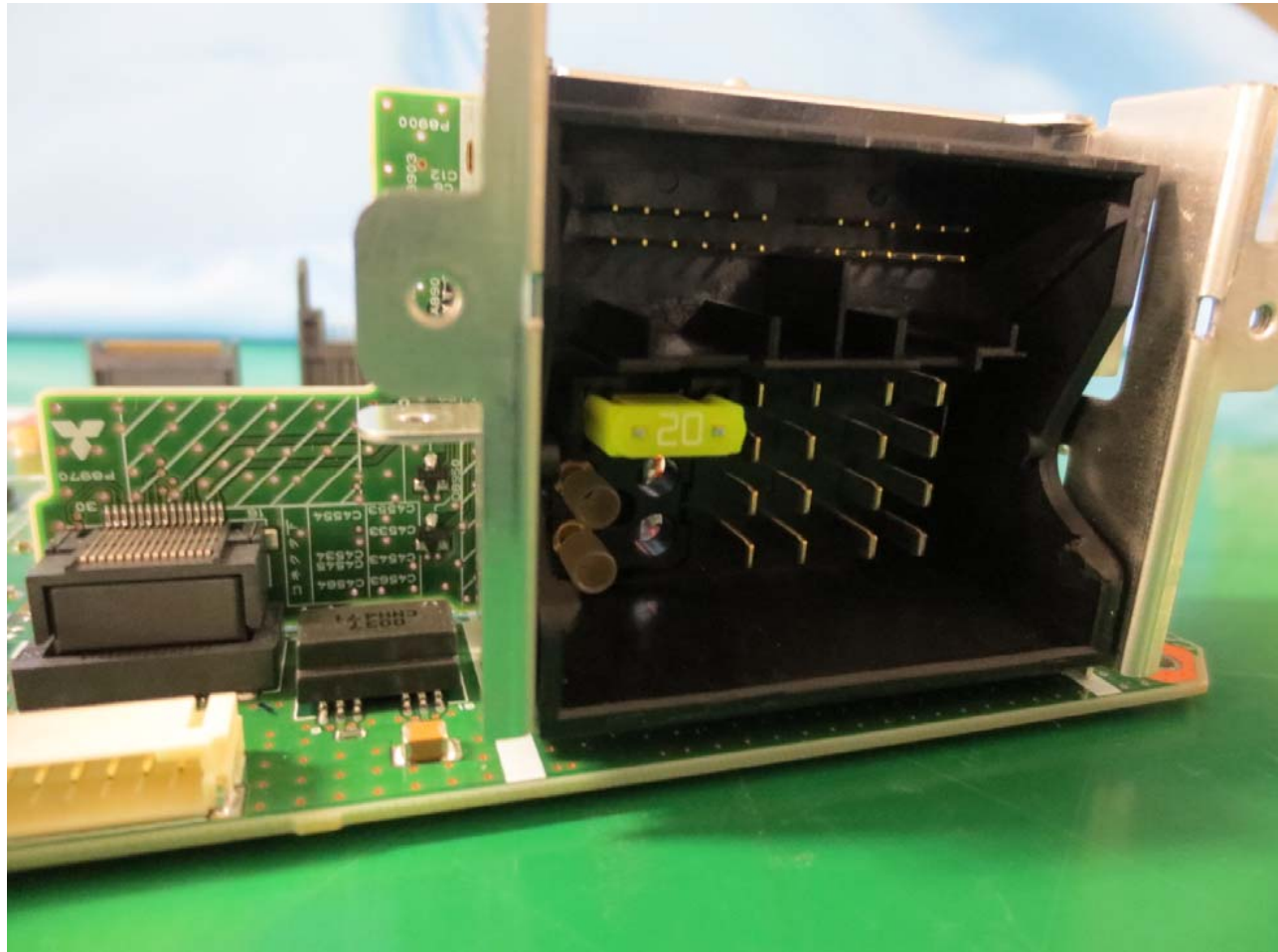
6. PCB-Combi S-side
