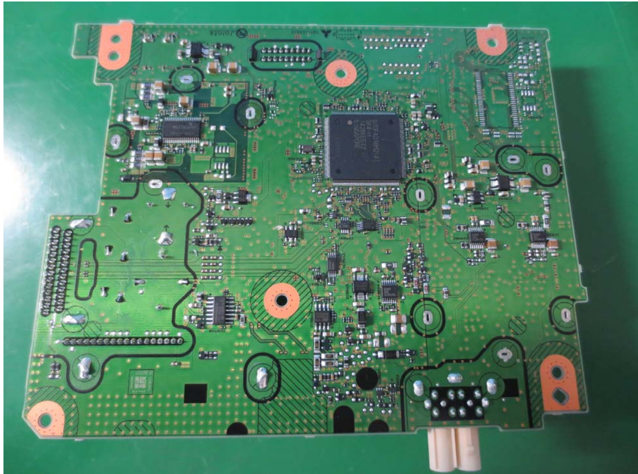
4. PCB-MAIN S-side
