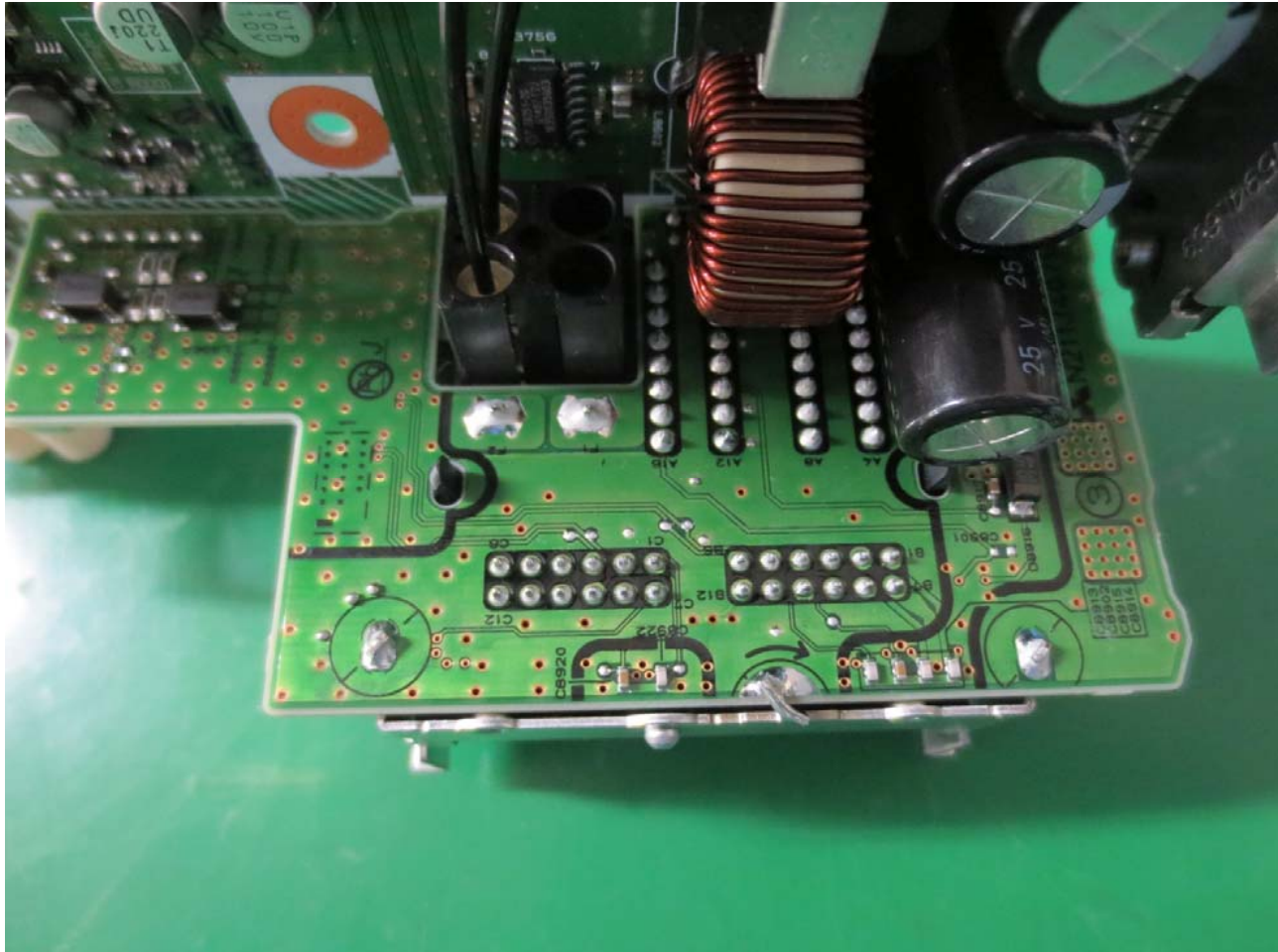
5. PCB-Combi C-side
