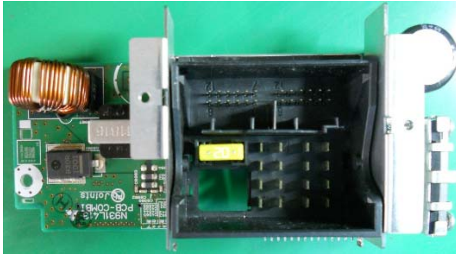
2. PCB-COMBI C-side
