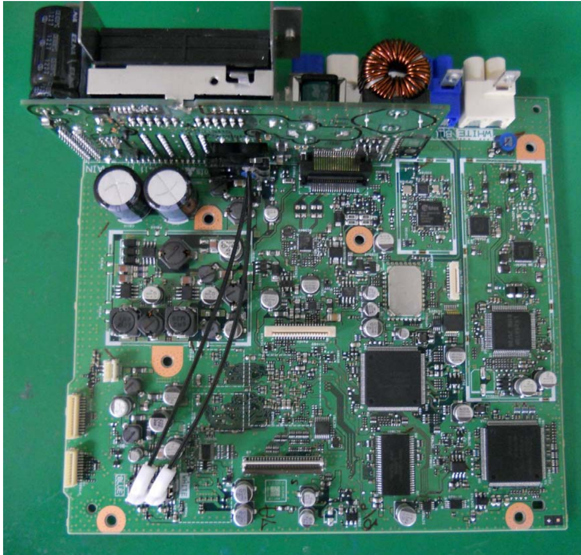
1. PCB-MAIN C-side
