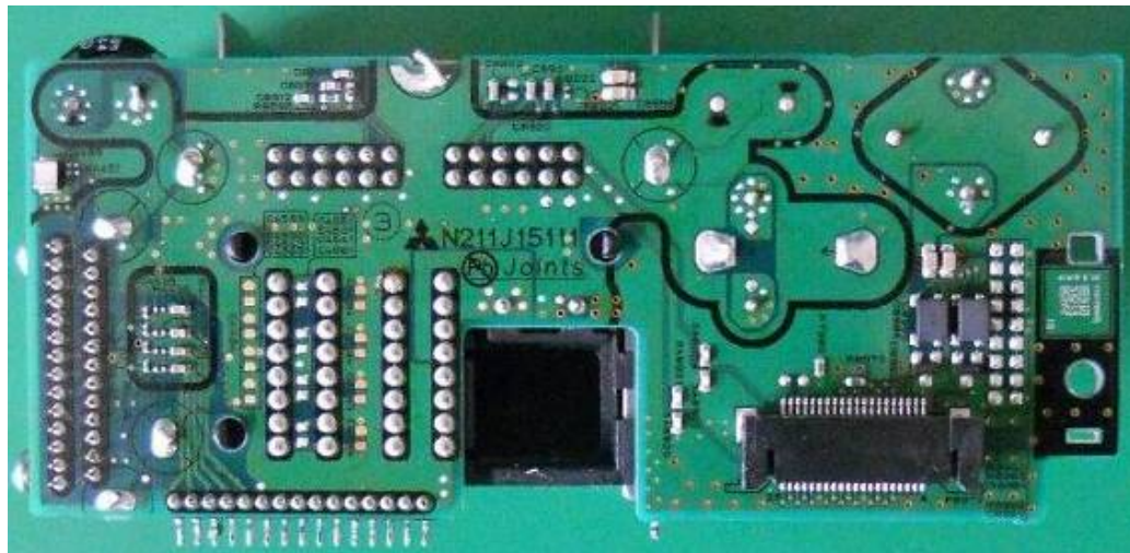
2. PCB-COMBI S-side
