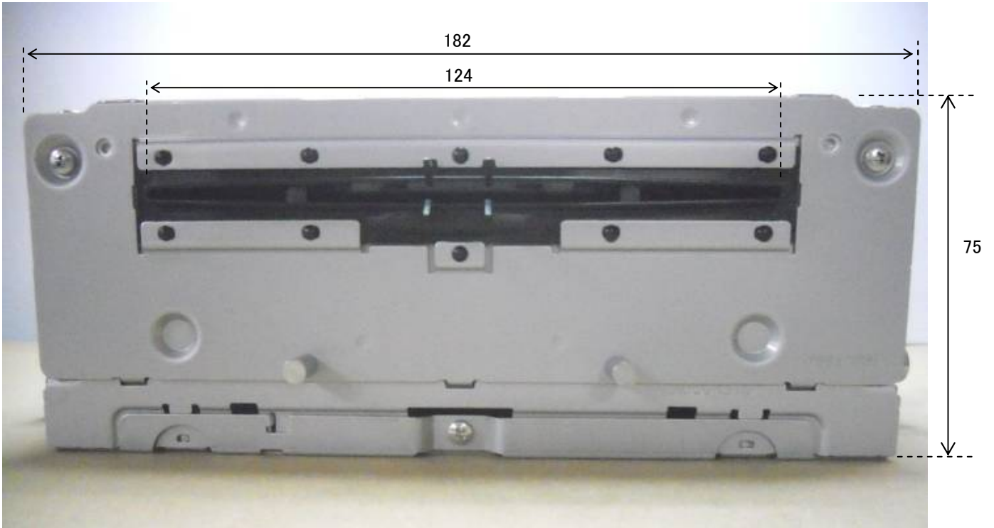
2. Front View
