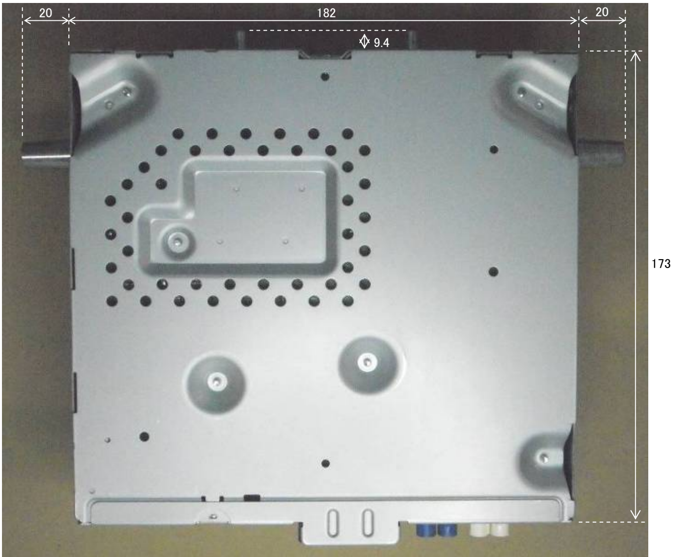
6. Bottom View
