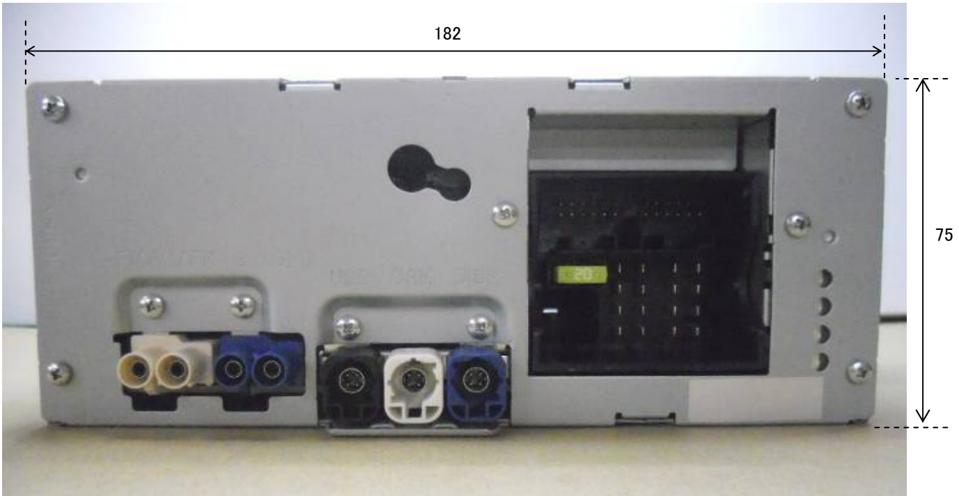
3. Rear View
