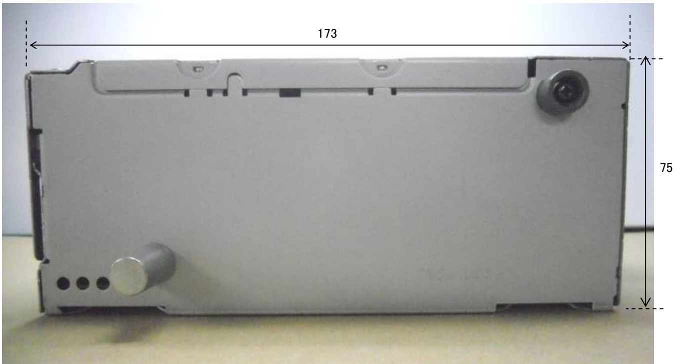
4. Right View
