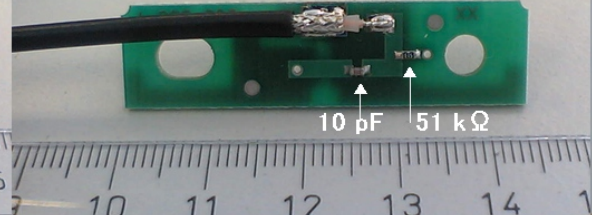
Bottom View of the Pattern Antenna
