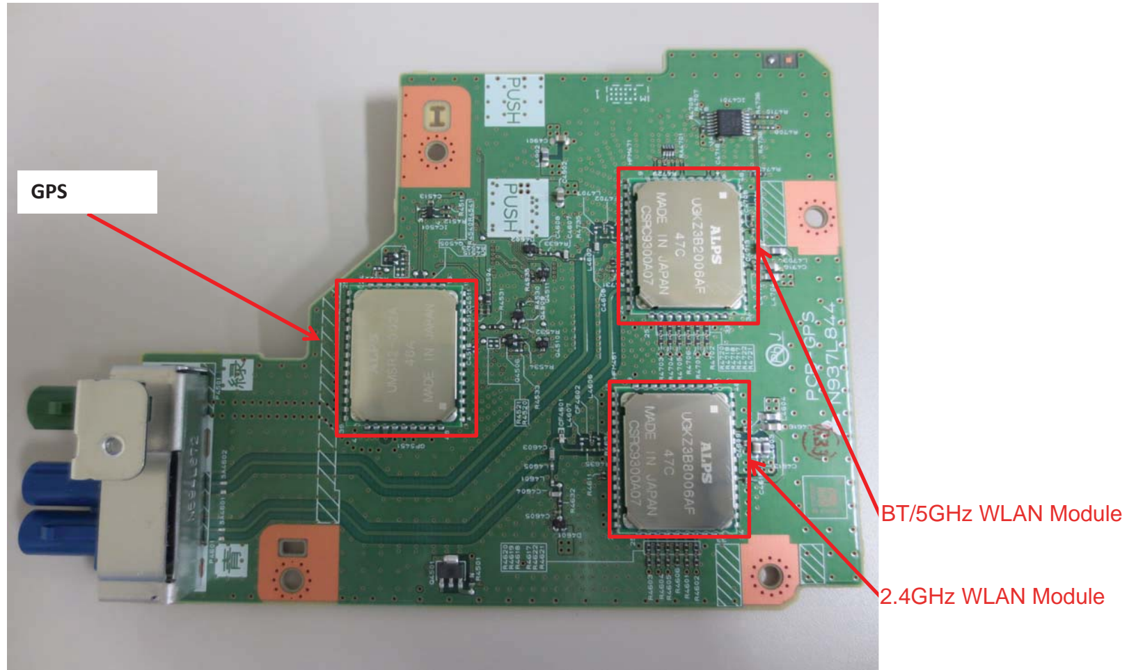
7. PCB-GPS C-side
