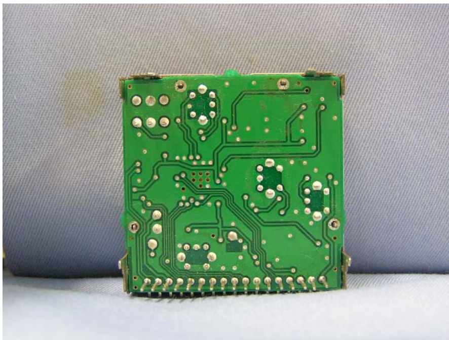
Solder side (TUNER PACK)
