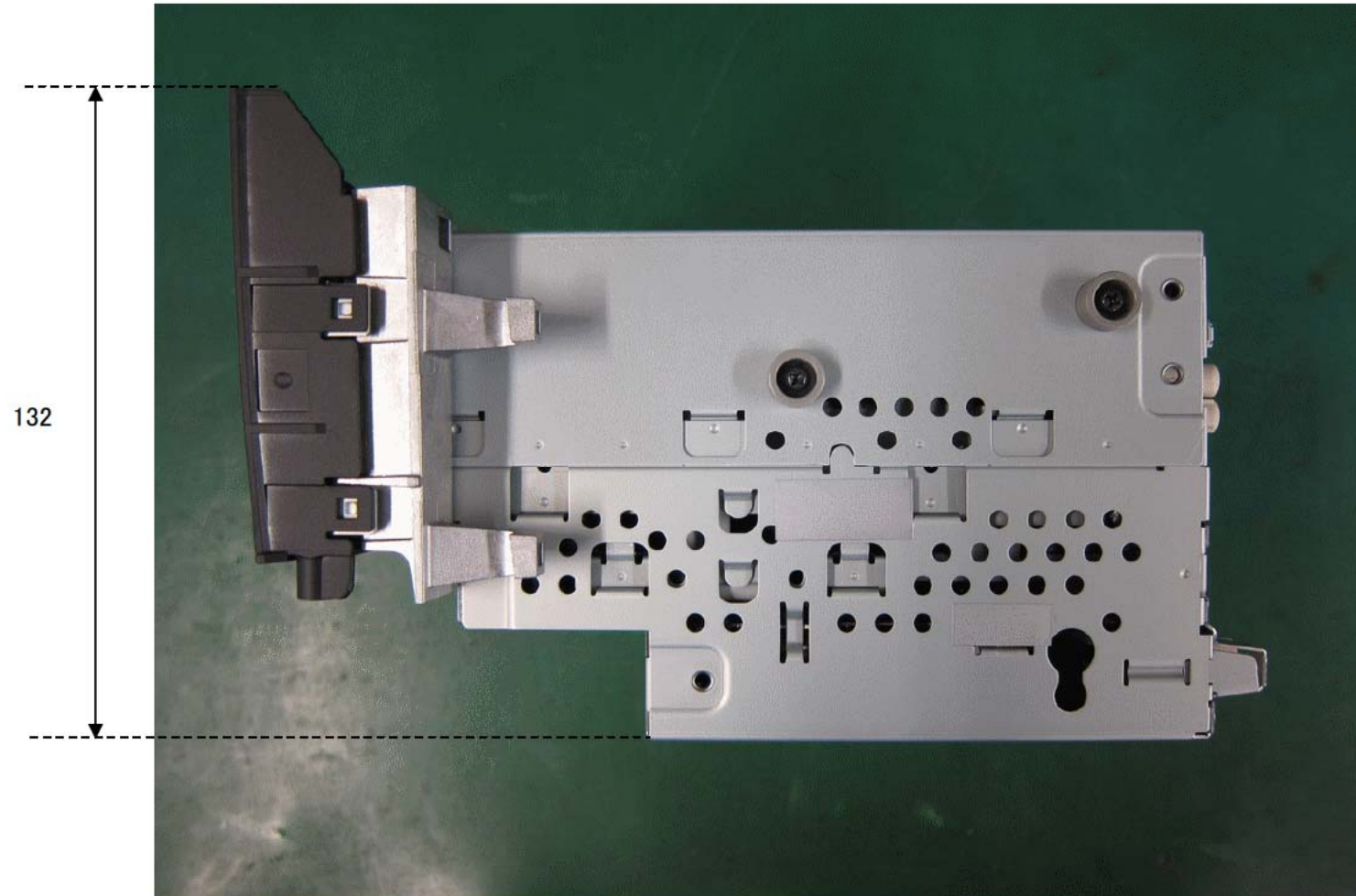
3. Right View
