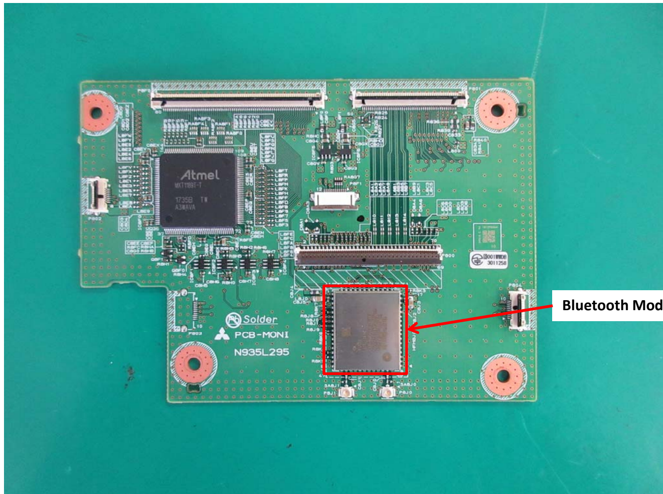
5. PCB-MONI C-side
