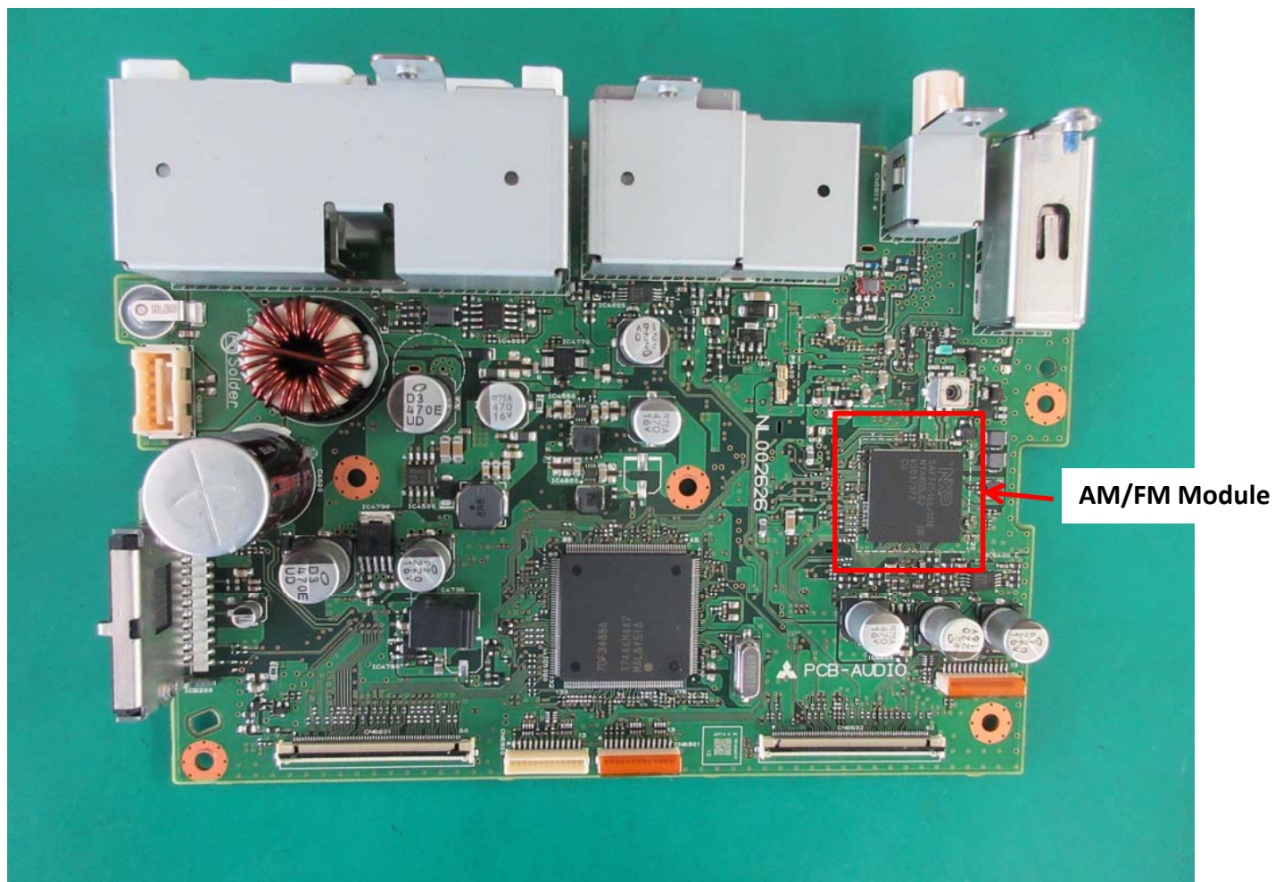
3. PCB-AUDIO C-side
