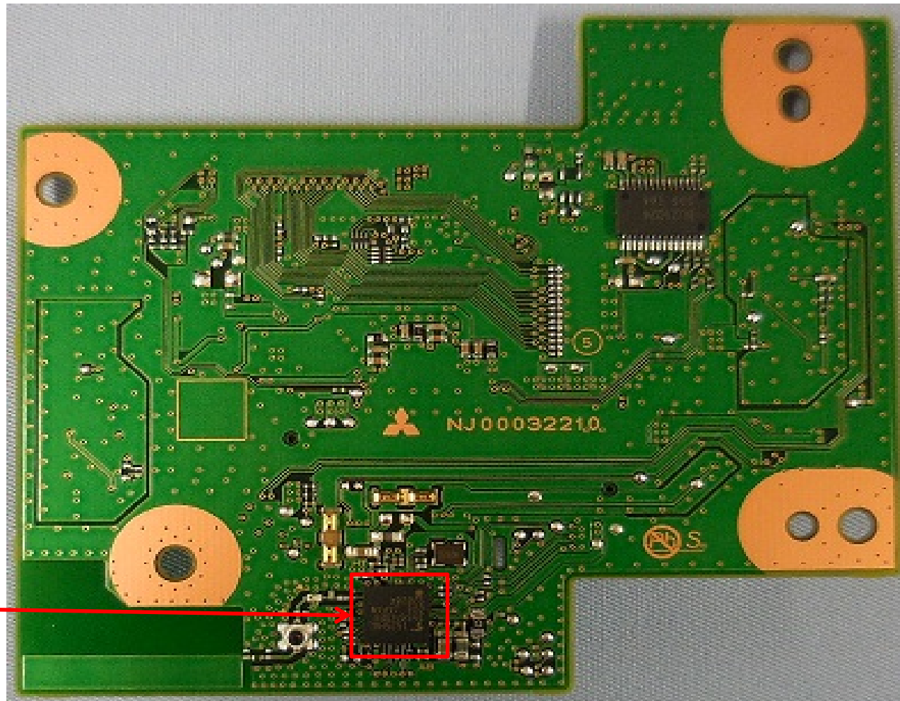
4. PCB-MONI S-side
