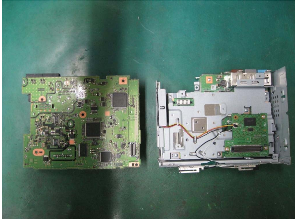
16. PCB-Main is removed. Copyright(c) Mitsubishi Electric Corporation
