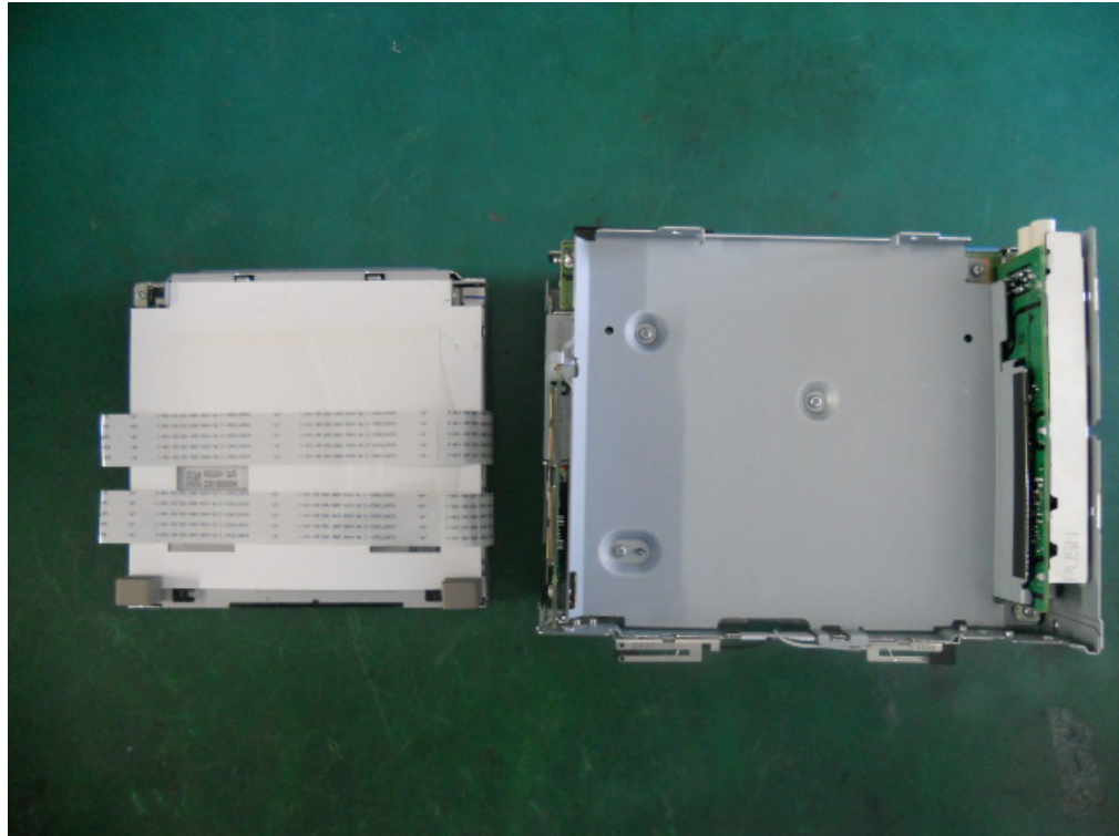
12. DVD drive is removed. Copyright(c) Mitsubishi Electric Corporation
