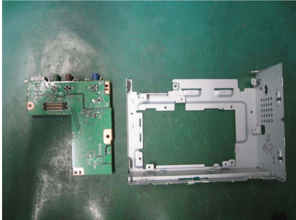
23. PCB-GPS is removed. Copyright(c) Mitsubishi Electric Corporation
