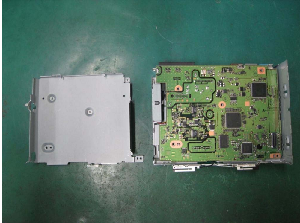
15. Internal plate is removed. Copyright(c) Mitsubishi Electric Corporation
