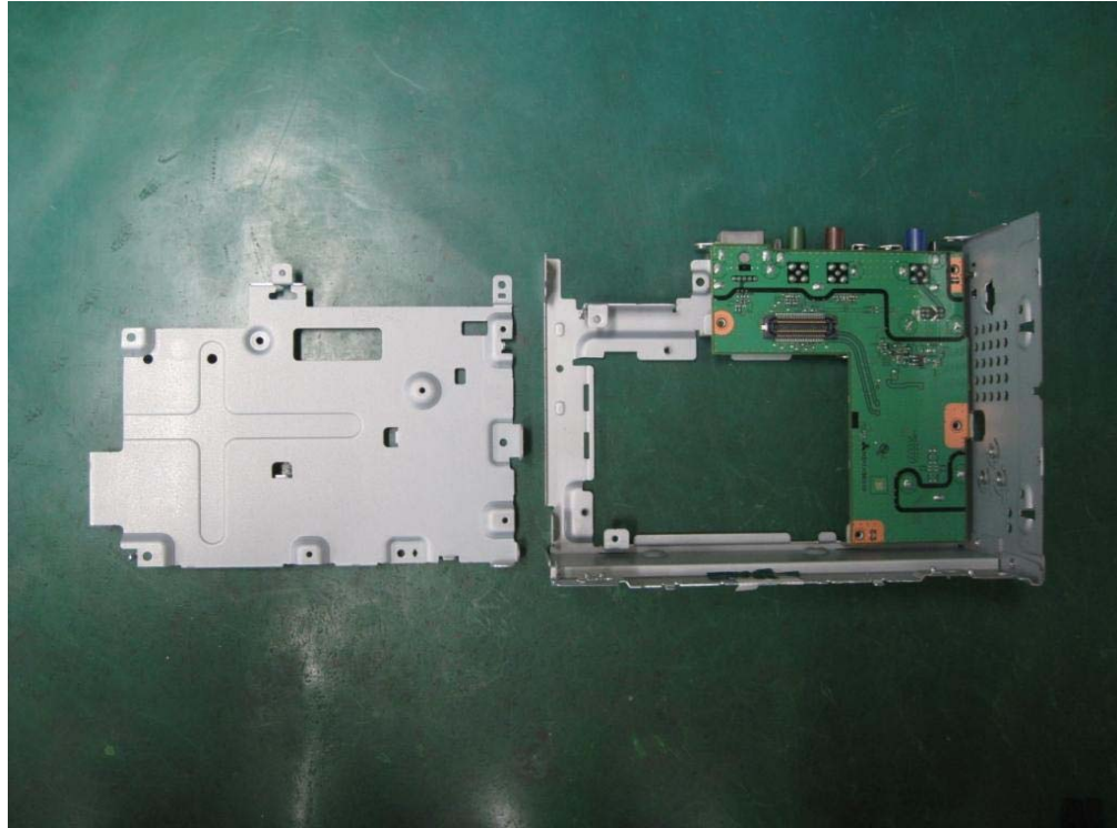
22. Internal plate is removed. Copyright(c) Mitsubishi Electric Corporation
