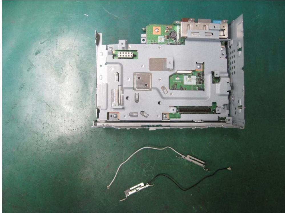
19. WLAN and Bluetooth antenna are removed. Copyright(c) Mitsubishi Electric Corporation
