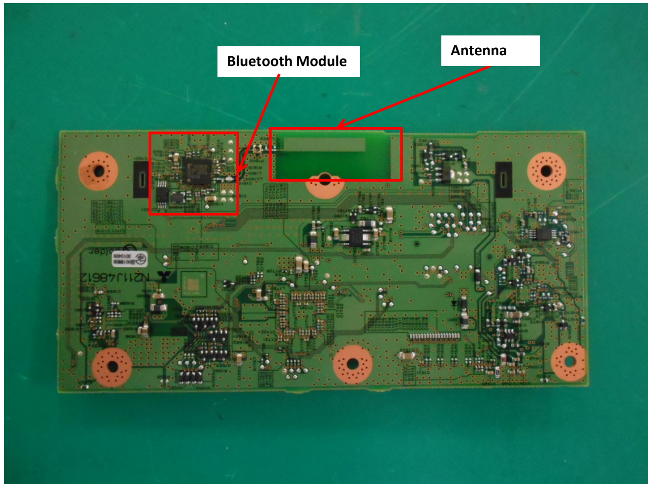
PCB-MONI S-side
