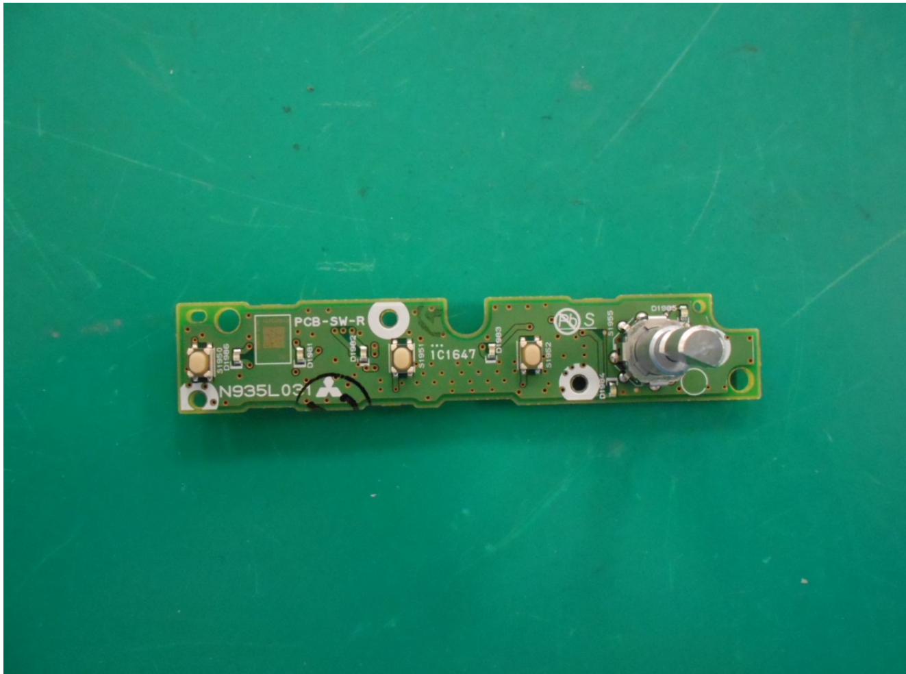
PCB-SW-R C-side
