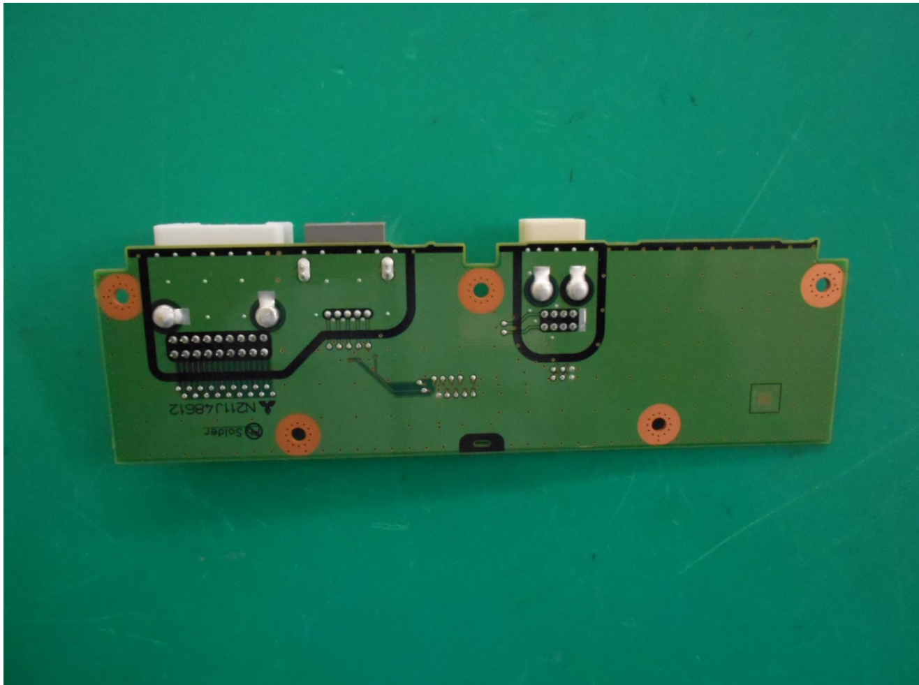
PCB-SUB S-side
