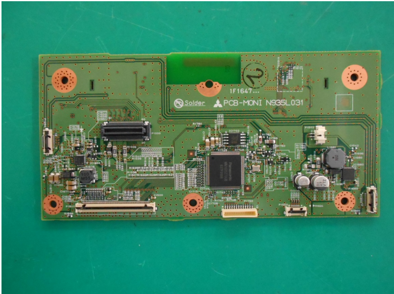
PCB-MONI C-side
