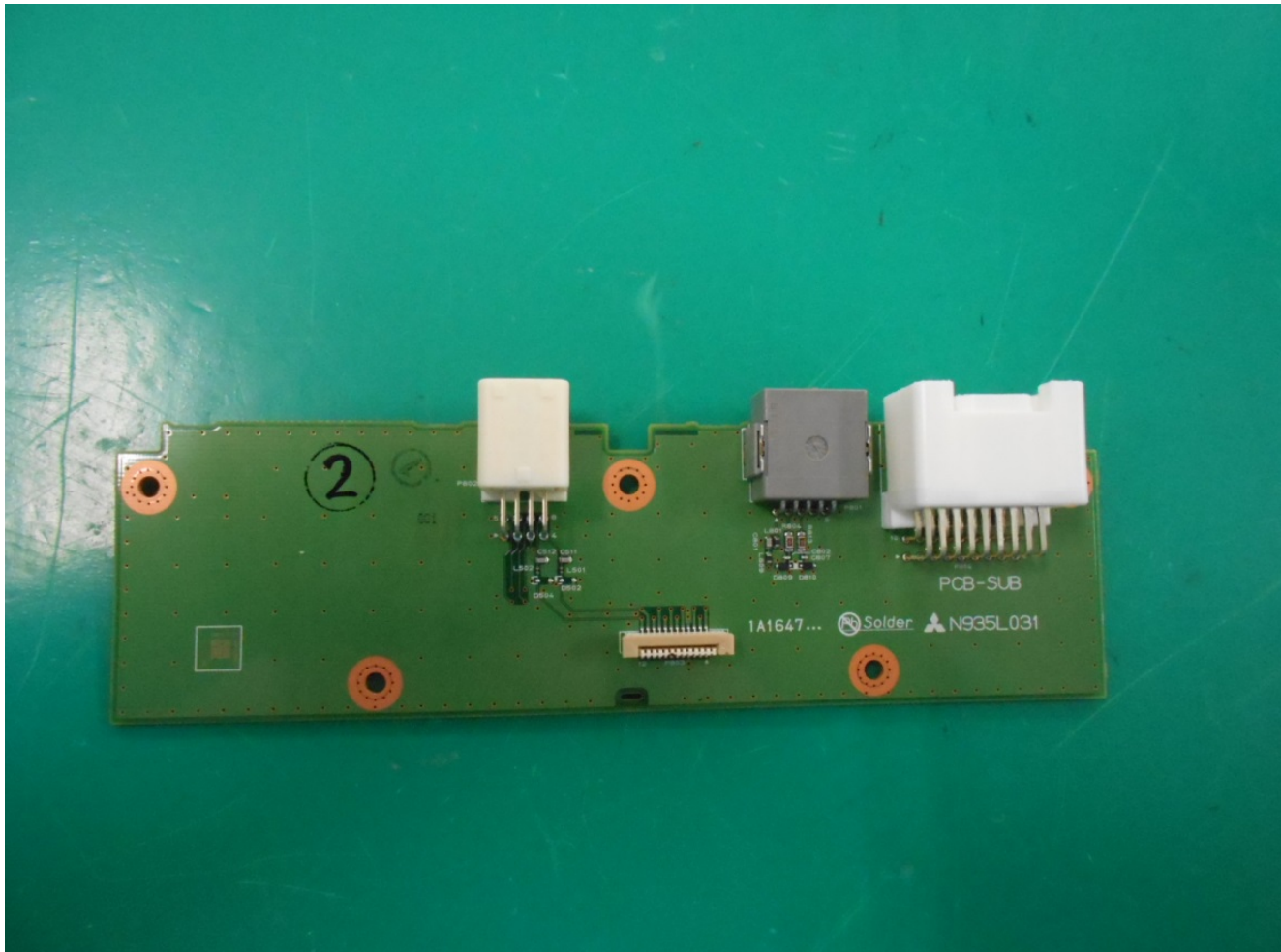
PCB-SUB C-side
