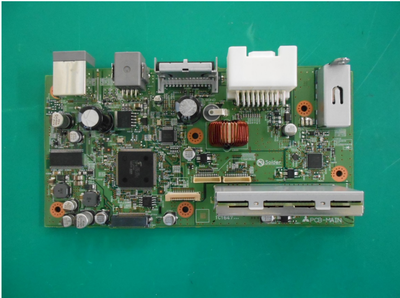
PCB-MAIN C-side
