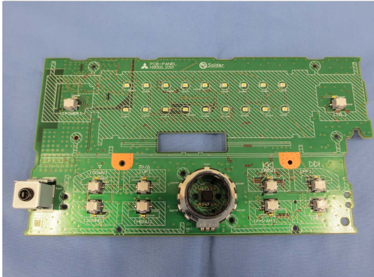
1. PCB-PANEL C-side
