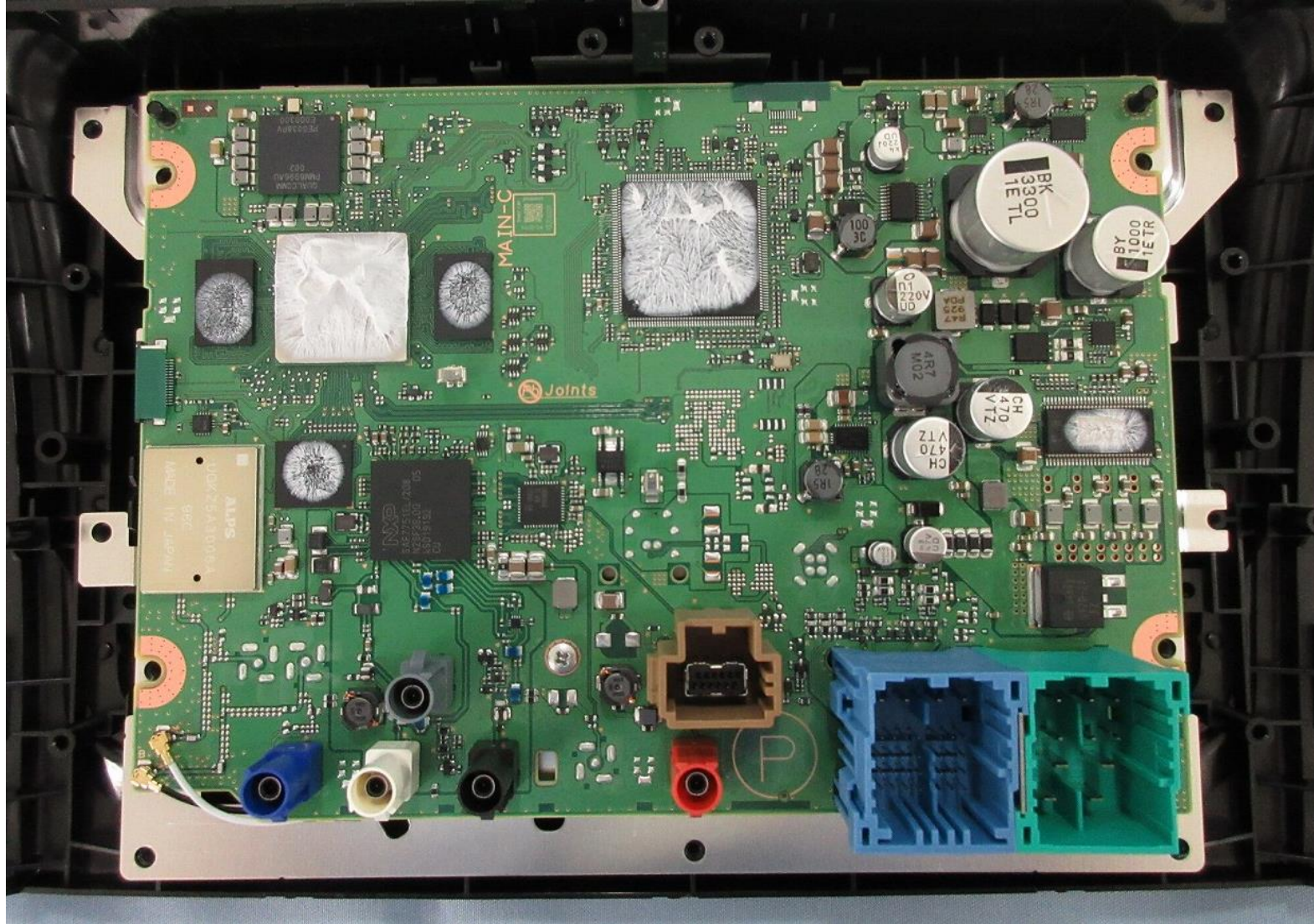
PCB-MAIN C-side
