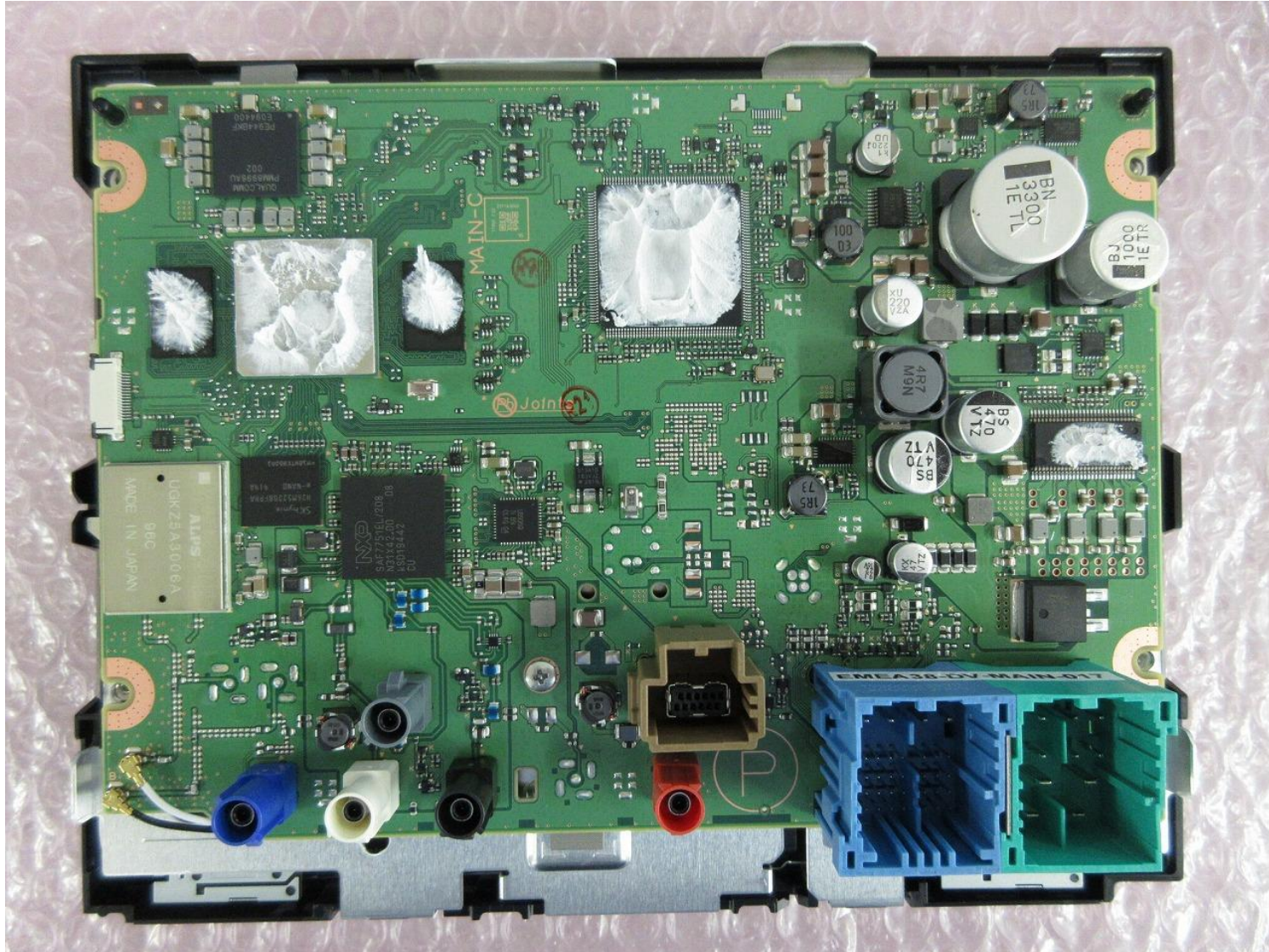
PCB-MAIN C-side
