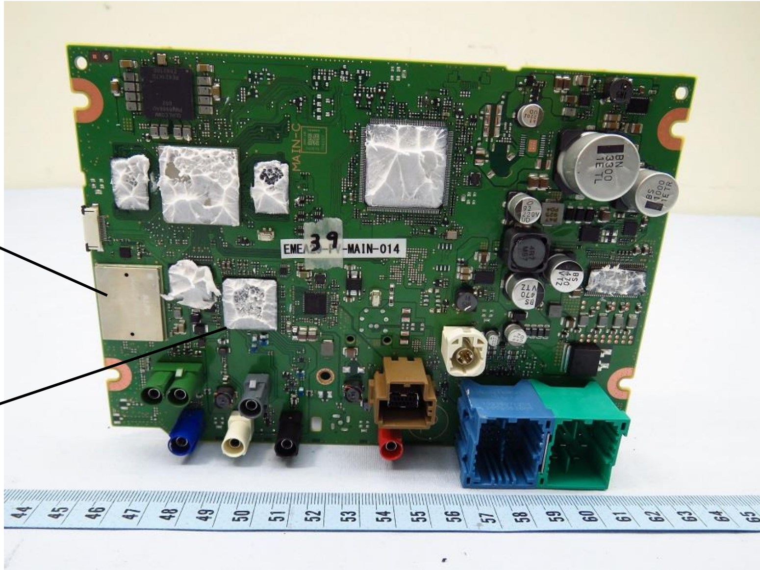
PCB-MAIN C-side
