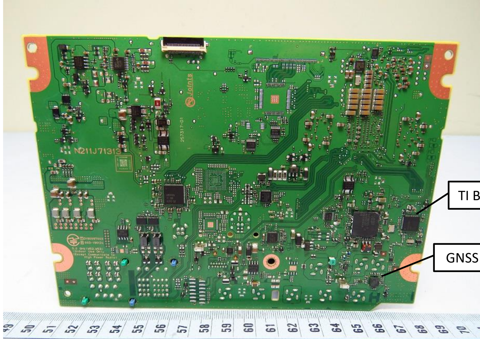
PCB-MAIN S-side
