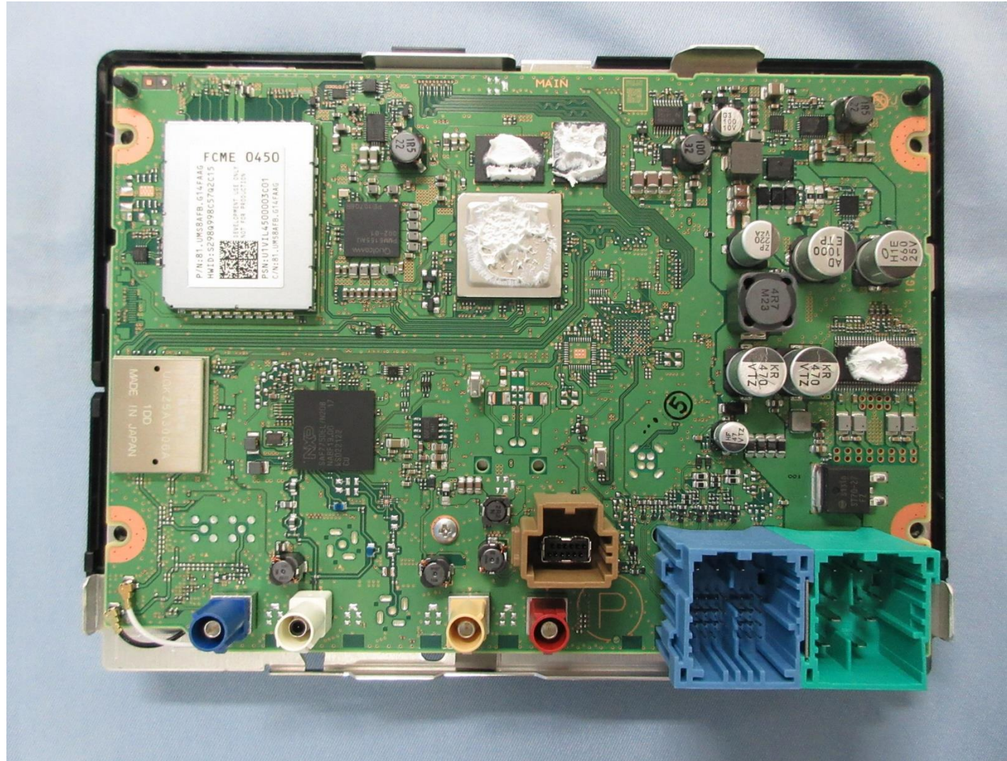
PCB-MAIN C-side
