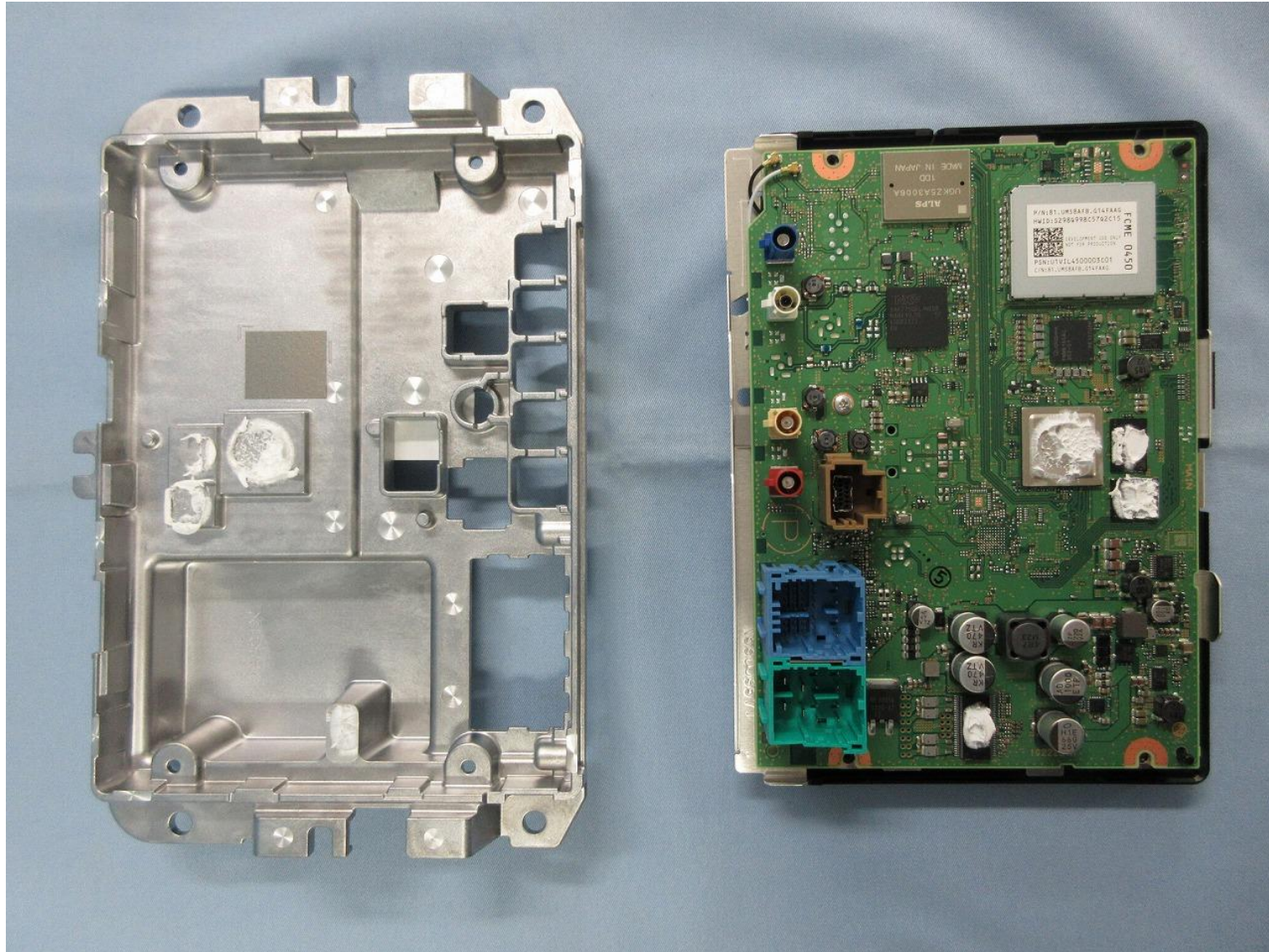
PCB-MAIN C-side
